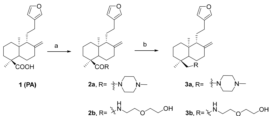
Scheme 1. Synthesis of PA derivatives. Reagents and conditions: (a) PPh 3 , amines, CCl 4 , 5 h, reflux; (b) DIBAL-H, THF, 4 h, RT.
