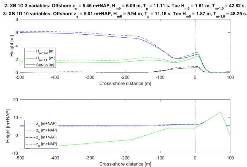
Figure 8. XBeach 1D calculations with 3 (solid lines) and 10 (dashed lines) stochastic variables at the design point. The dike toe is indicated by the dotted line. The parameters offshore and at the toe of the dike are given in the title of the figure.
