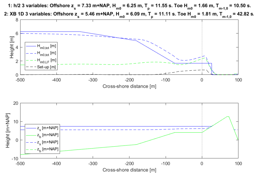
Figure 7. h/2 -model (solid lines) versus XBeach 1D (dashed lines) with the offshore conditions as stochastic variables and a morphostatic foreshore at the design point. The dike toe is indicated by the dotted line.
