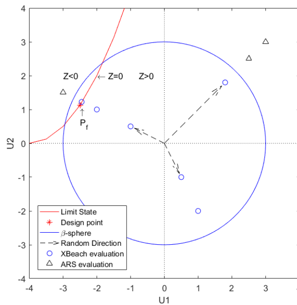
Figure 3. A schematized and arbitrary example of the ADIS method, with two stochastic variables (U1 and U2). The standard normal space is given, together with the limit state (red line), the design point (red asterisk), \beta -sphere (blue circle), random directions (dashed arrows) and XBeach and ARS evaluations (blue circles and black triangles). The areas where Z < 0 and Z > 0 and the limit state Z = 0 are indicated as well (after Den Bieman et al.; Grooteman [21,36]).
