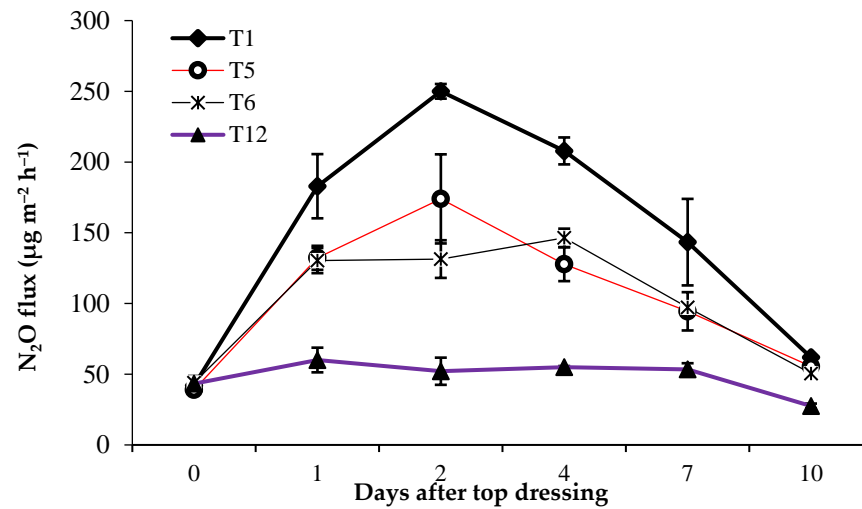
Figure 4. The mean N_2O flux ( \mu\text{g m}^{-2} \text{h}^{-1} ) and Days after top dressing (DATD) [over 2 years] are influenced by various treatments. [T1 = STB-based NPK application; T5 = RDF (120-60-40 NPK/ha); T6= Nutrient Expert based (LCC) NPK & T12 = STB-based N_0 PK application]. Each bar for treatment shows the standard error of the mean ( \text{SEM} \pm ), which was calculated for each treatment for three replications.
