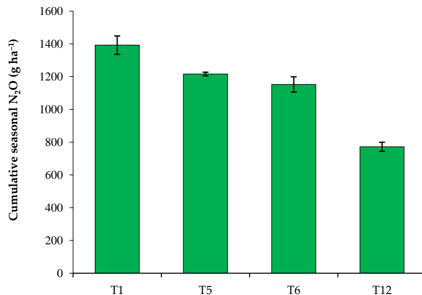
Figure 5. Cumulative seasonal mean N_2O ( \text{g ha}^{-1} ) emission over various treatments [over 2 years]. [Where T1 = STB-based NPK application; T5 = RDF (120-60-40 NPK/ha); T6 = Nutrient Expert based (LCC) NPK & T12 = STB-based N_0 PK application]. Each bar for treatment shows the standard error of the mean ( \text{SEM} \pm ), which was calculated for each treatment for three replications.
