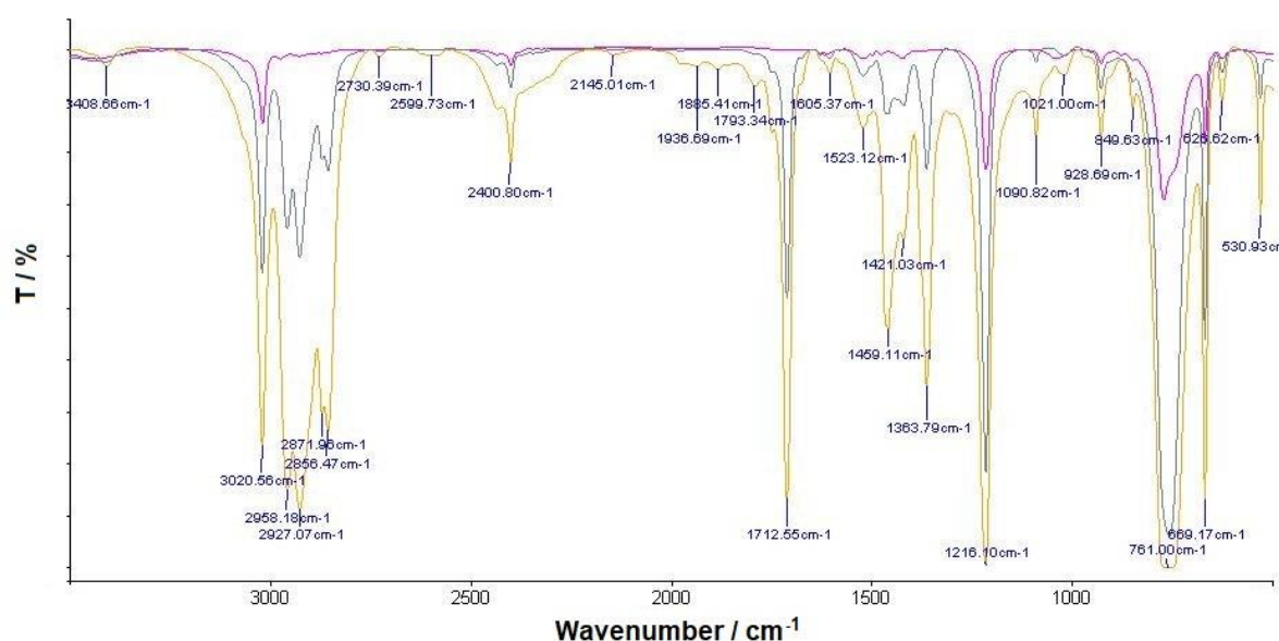
Figure S1. FTIR spectra of extracts after first (yellow), second (grey) and third (pink) cleaning cycle.
