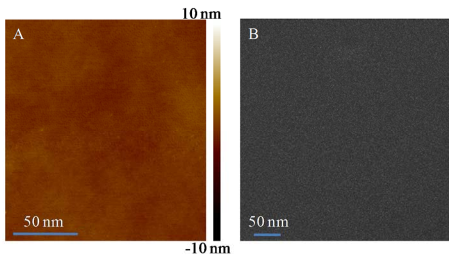
Figure S1. The images of nanoplate film after 15 minutes deposited on untreated silicon surface ( A ) AFM image ( B ) FESEM image.
