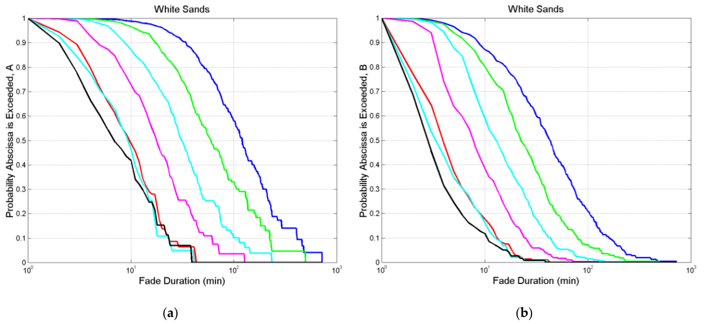
Figure A7. White Sands. (a) Probability distribution P_{S,A}(D) of exceeding the value indicated in abscissa at the following thresholds: 0 dB, blue; 3 dB, green; 6 dB, cyan; 10 dB, magenta; 20 dB, red; 29~40 dB, cyan and black; (b) P_{S,B}(D) , same legend.
