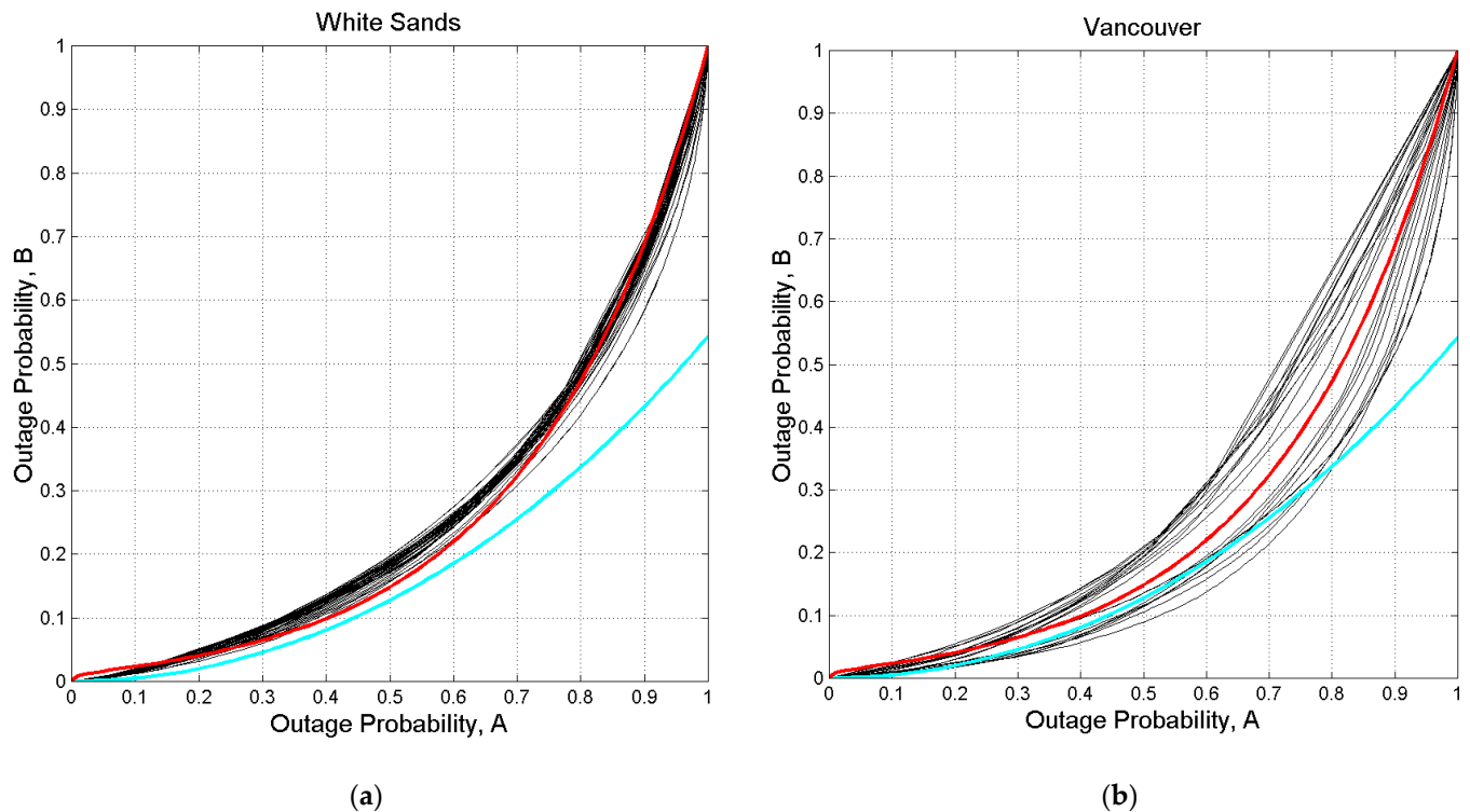
Figure A15. P_{S,B}(D) ( y -axis) versus P_{S,A}(D) ( x -axis), 80 GHz, circular polarization, zenith paths: (a) White Sands, for thresholds from 0 to 40 dB; (b) Vancouver, for thresholds from 0 to 20 dB. The red line is drawn from Equation (3); the cyan line is drawn from Equation (5).
