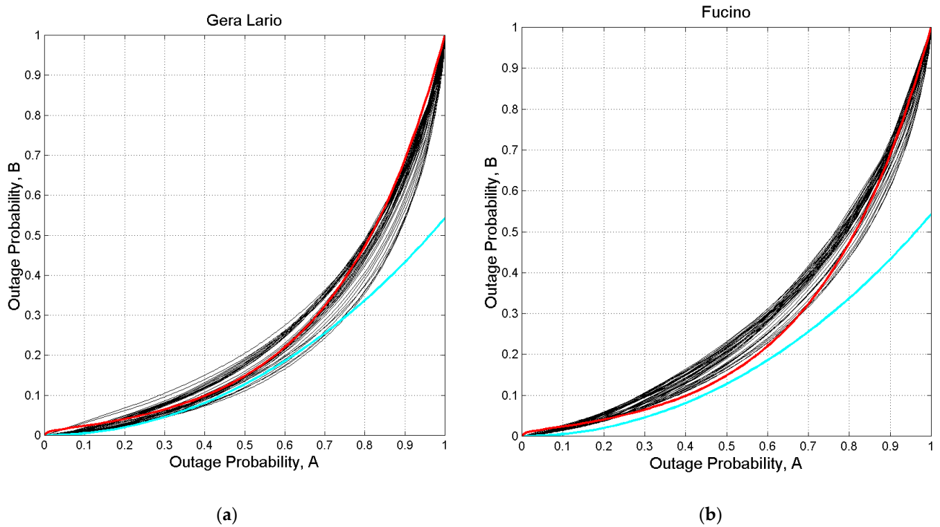
Figure A12. P_{S,B}(D) (y-axis) versus P_{S,A}(D) x-axis, for thresholds from 0 to 40 dB, 80 GHz, circular polarization, zenith paths: (a) Gera Lario; (b) Fucino. The red line is drawn from Equation (3); the cyan line is drawn from Equation (5).
