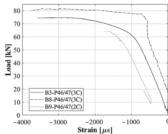
Figure 17. Applied load versus top compressive strain.
