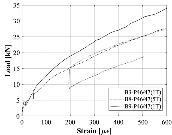
Figure 16. Applied load versus crack reopening.
