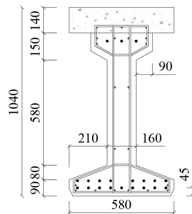
Figure 3. I-beam cross-section (in mm).
