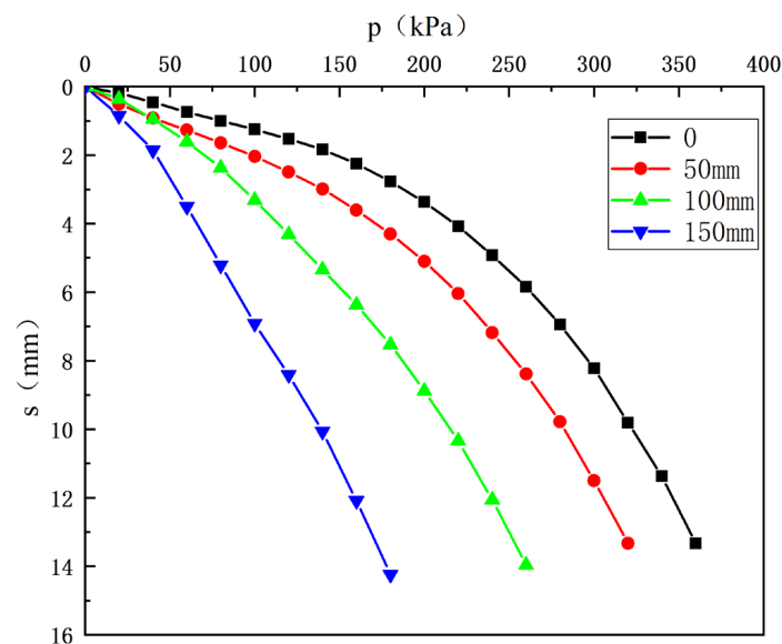
Figure 4. The p - s curves at different water levels.
