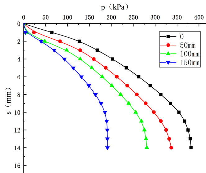
Figure 13. The p – s curves for different water-level heights.
