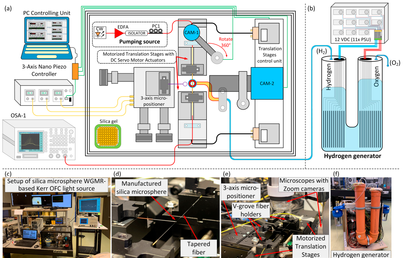
Figure 2. (a) Experimental setup illustrating the developed silica microsphere WGMR-based Kerr-OFC as a light source for optical communications. (b) Schematic of a Hydrogen generator for pure generation of hydrogen ( H_2 ) and oxygen ( O_2 ) by electrolysis of water. (c) Captured setup of silica microsphere WGMR-based Kerr-OFC light source. (d) Tapered fiber and silica microsphere resonator positions inside of enclosure box for dust and airflow prevention. (e) The 3-axis X, Y, and Z micro-positioner stage with a built-in Piezo controller and compact, motorized translation stages together with zoom microscopes used to monitor the position of the WGMR resonator. (f) Captured hydrogen generator for pure hydrogen and oxygen production.
