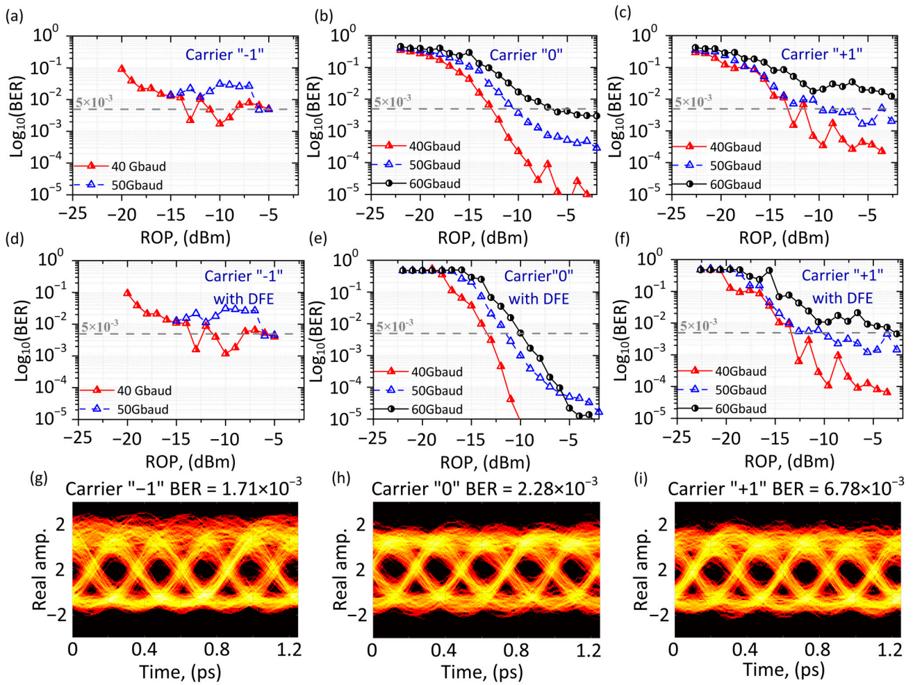
Figure 8. BER versus ROP for the IM/DD communication system where the Kerr-OFC light source carriers “−1”, “0”, and “+1” can be used for NRZ-OOK signals transmission with baud rates up to (a) 50 Gbaud, (b) 60 Gbaud, and (c) 50 Gbaud without any post-equalization. If the post-equalizer with 33-FF and 15-FB taps is used, the BER is significantly improved for carriers “−1”, “0”, and “+1” up to (d) 50 Gbaud, (e) 60 Gbaud, and (f) 60 Gbaud. Received signal eye diagrams for carriers: (g) “−1”, (h) “0”, and (i) “+1” captured at ROP of −10 dBm in the 40 Gbaud case.
