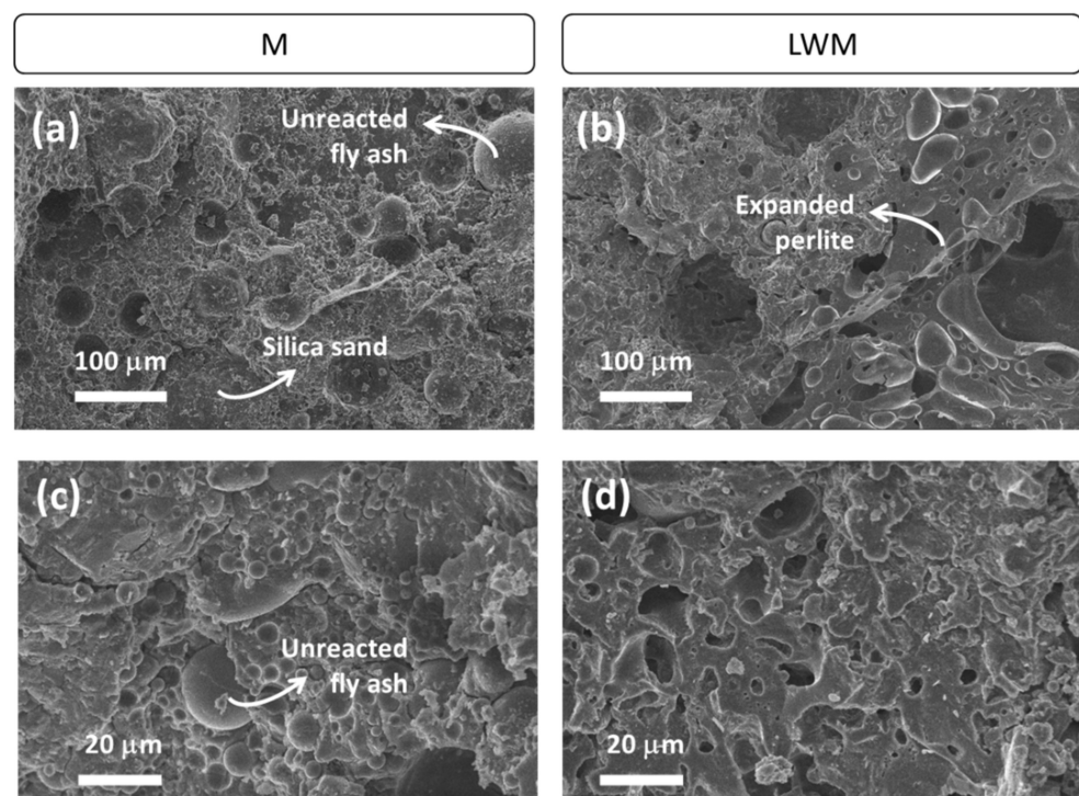
Figure 4. SEM morphological observation of (a,c) M and (b,d) LWM samples at different magnifications: (a,b) at 200 \times and (c,d) at 1000 \times .
