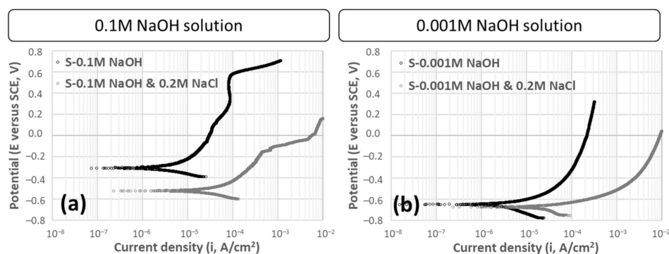
Figure 9. Anodic polarization curves of sand blasted steel (S) in (a) 0.1 M NaOH and (b) 0.001 M NaOH aqueous solutions without and with the addition of 0.2 M NaCl.
