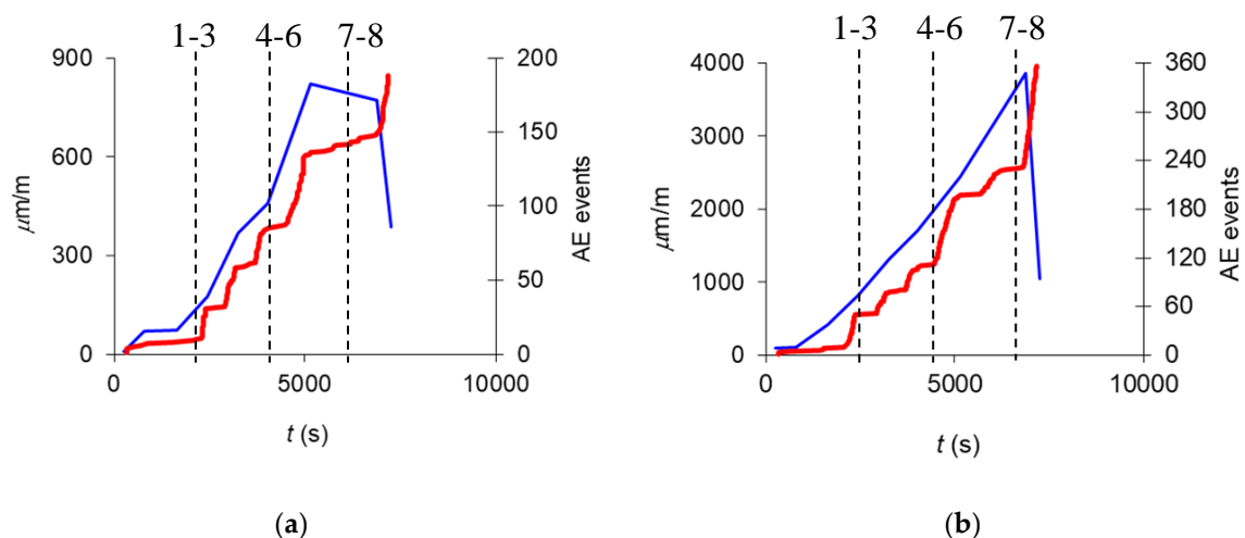
Figure 12. Cumulative AE activity (red) and FOS strain (blue) time histories for: (a) fiber optic n.9 at x = -1.6\text{ m} and AE sensor n.4; (b) fiber optic n.9 at x = -1.2\text{ m} and AE sensor n.5. The dashed lines identify the different loading stages.
