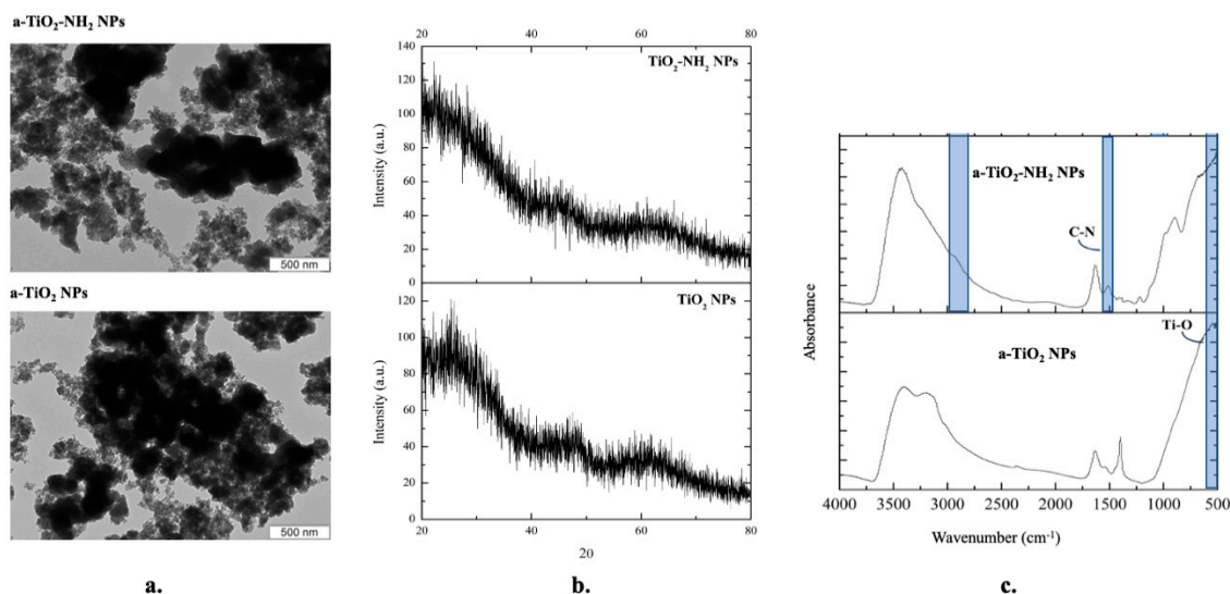
Figure 1. Physical characterization of amorphous TiO 2 (a-TiO 2 ) (lower panels) and a-TiO 2 -NH 2 nanoparticles (NPs) (upper panels): (a) TEM images, (b) X-ray diffractograms, and (c) FTIR spectra.
