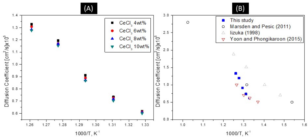
Figure 3. (A) Diffusion coefficient of Ce^{3+} as a function of CeCl_3 concentration and temperature in LiCl-KCl. (B) Comparison of values from literature.
