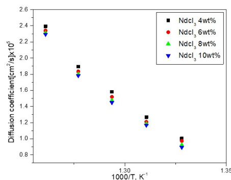
Figure 6. Diffusion coefficient changes as a function of NdCl 3 concentration in LiCl-KCl.
