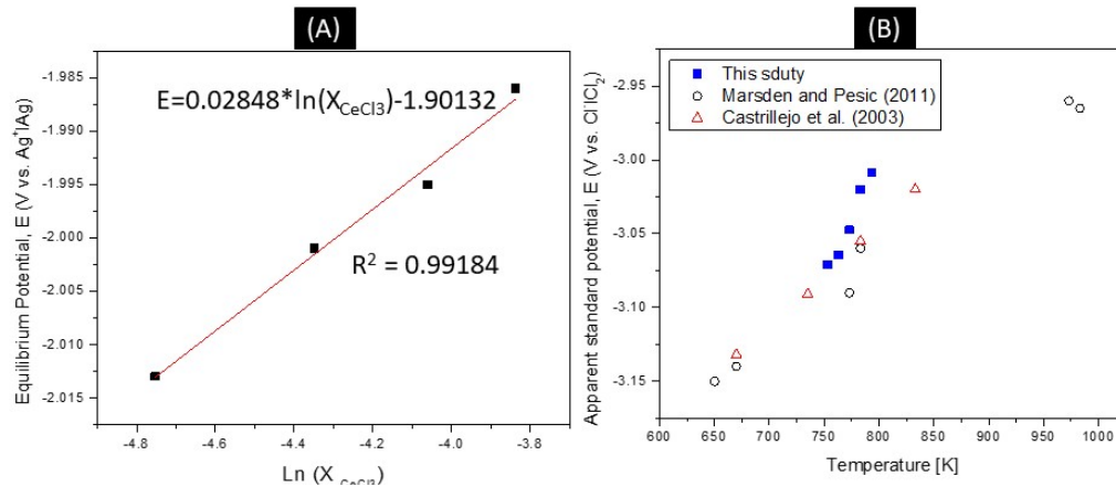
Figure 8. (A) -1.901 V apparent standard potential vs. the 5 mol% Ag^+/Ag reference scale at 773 K. (B) Comparison of values from literature [7,14].
