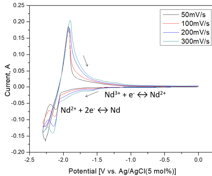
Figure 5. Cyclic Voltammograms of 4 wt% NdCl 3 in LiCl-KCl eutectic molten salt with scan rate; 50, 100, 200, 300 mV/s at 773 K.
