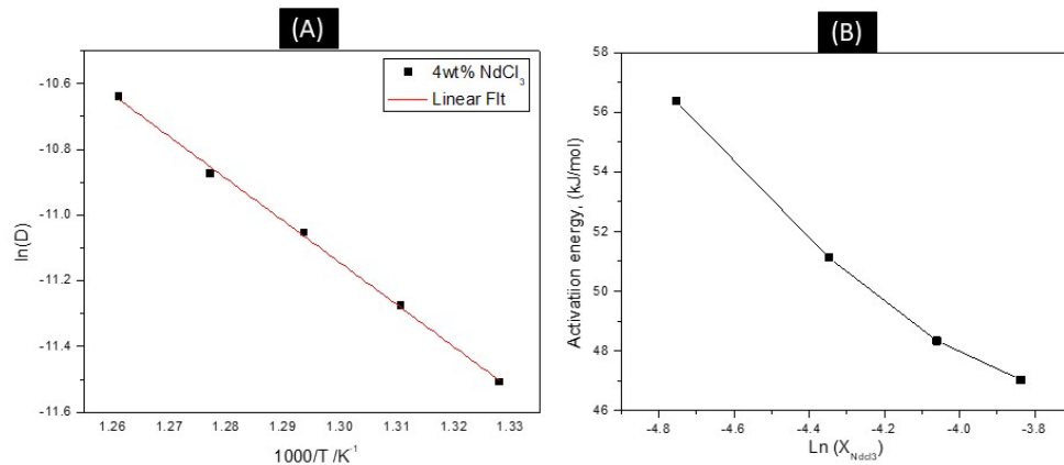
Figure 7. (A) Linear relationship of the logarithm of \text{NdCl}_3 diffusion coefficient vs. the reciprocal of absolute temperature. (B) Activation energy as a function of \text{NdCl}_3 concentration.
