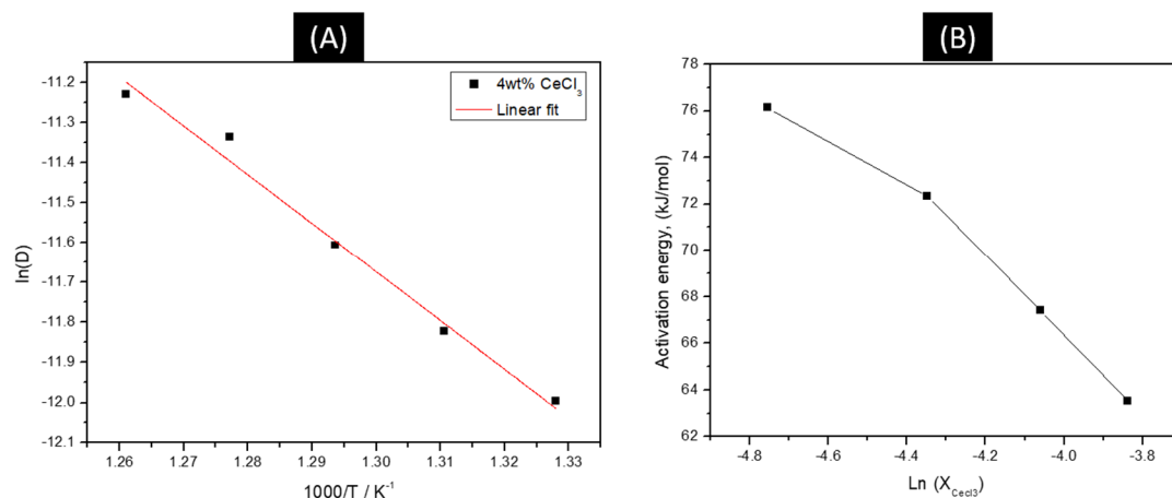
Figure 4. (A) Linear relationship of the logarithm of CeCl_3 diffusion coefficient vs. the reciprocal of the absolute temperature. (B) Activation energy as a function of CeCl_3 concentration.
