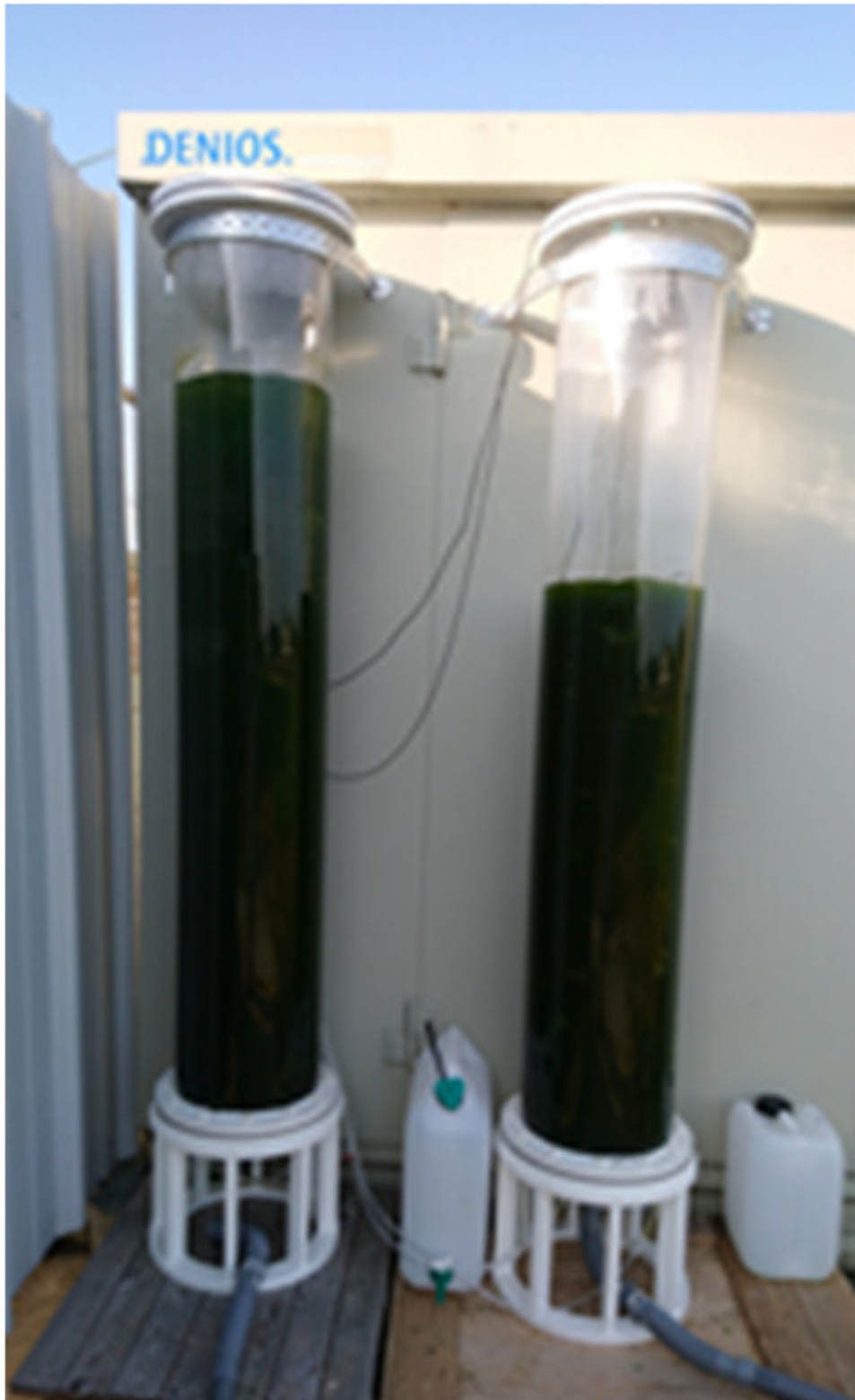
Figure 2. Cultivation of Monoraphidium sp. in photobioreactors of 110L in batch/ semi-continuous regimes with digestate diluted at 1:50.
