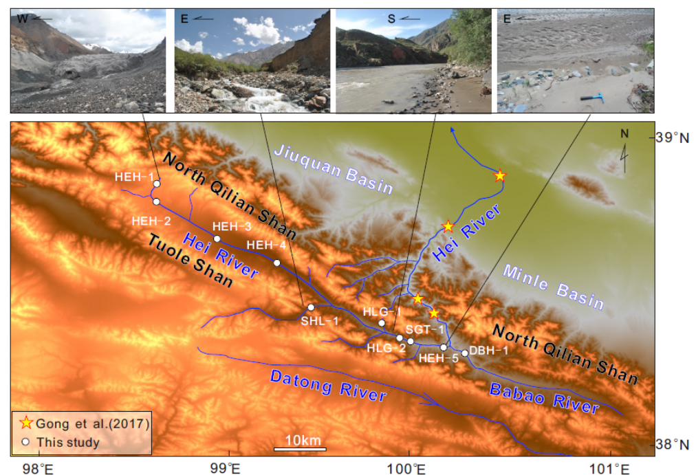
Figure 6. Sampling locations for available detrital zircon U-Pb (stars, [90]) and ZFT (circles, this study) data in the Hei River drainage. The color of the stars and circle refer to the different studies.
