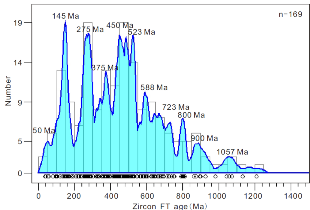
Figure 7. Kernel analysis histogram of all individual ZFT ages obtained from the Hei River. Calculated using the Density Plotter software (Version 8.5, Vermeesch, P, London, UK, https://www.ucl.ac.uk/~ucfbpve/densityplotter/ , accessed on 25 February 2022) [104]. Raw analytical data are available as “Supplement Table S1” to this article.
