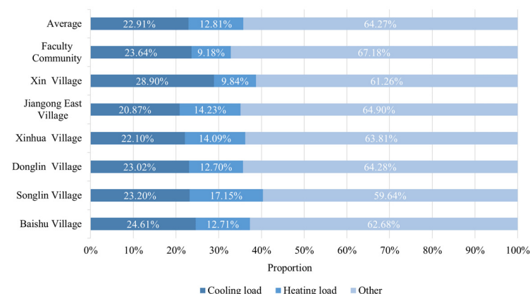
Figure 9. Statistical results of the energy for cooling and heating proportions of each residential district.
