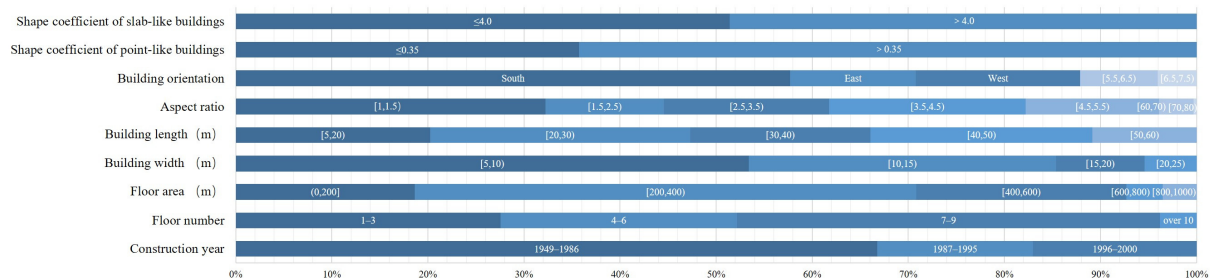
Figure 5. Statistical analysis of the form characteristics of sample buildings.
