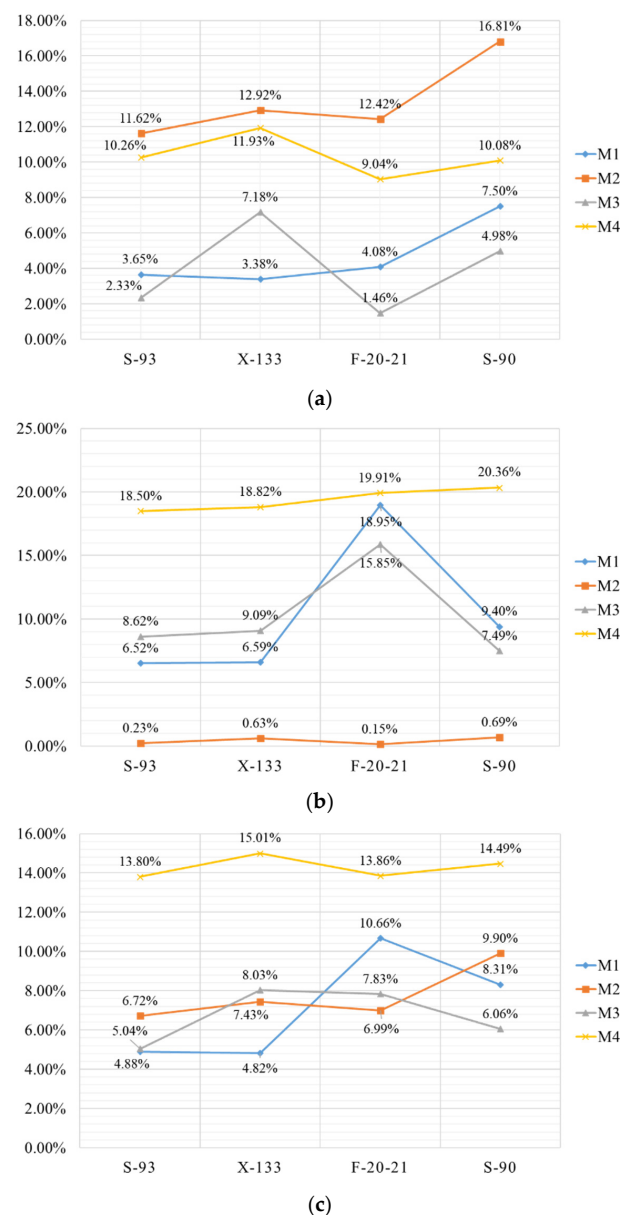
Figure 13. Comparison of energy-saving measures: (a) is the energy-saving rate on cooling energy consumption; (b) is the energy-saving rate on heating energy consumption; and (c) is the energy-saving rate on overall energy consumption.
