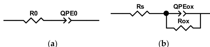
Figure 10. Equivalent circuit used to model EIS data of the AS sample: (a) at the beginning of the test (0 h) and (b) for a prolonged time of immersion.
