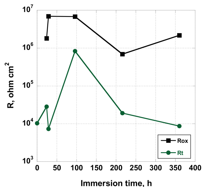
Figure 16. Variation of R_{ox} and R_t as a function of time of immersion in Hank's solution displayed by the NT sample.
