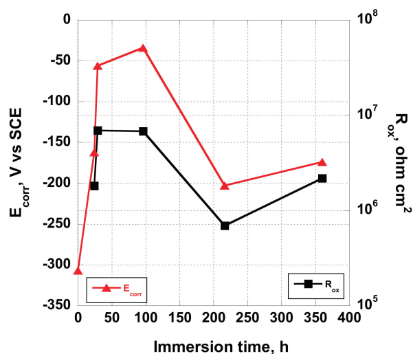
Figure 11. Variation of E_{\text{corr}} and R_{\text{ox}} as a function of time of immersion in Hank's solution displayed by the AS sample.
