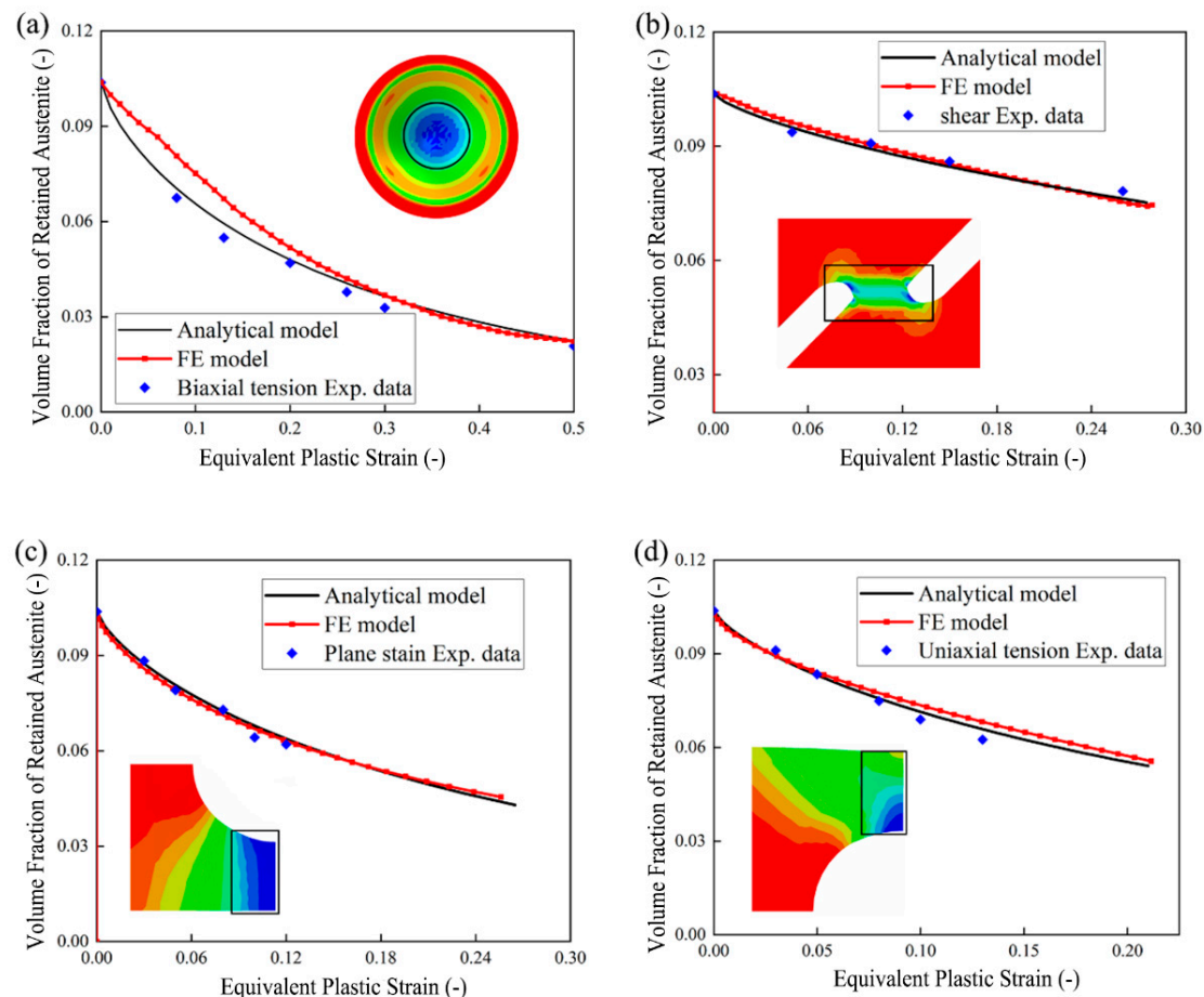
Figure 10. Comparisons of the VFRA using analytical and FE model: (a) Nakajima specimen; (b) shear specimen; (c) notched specimen; (d) central hole specimen.
