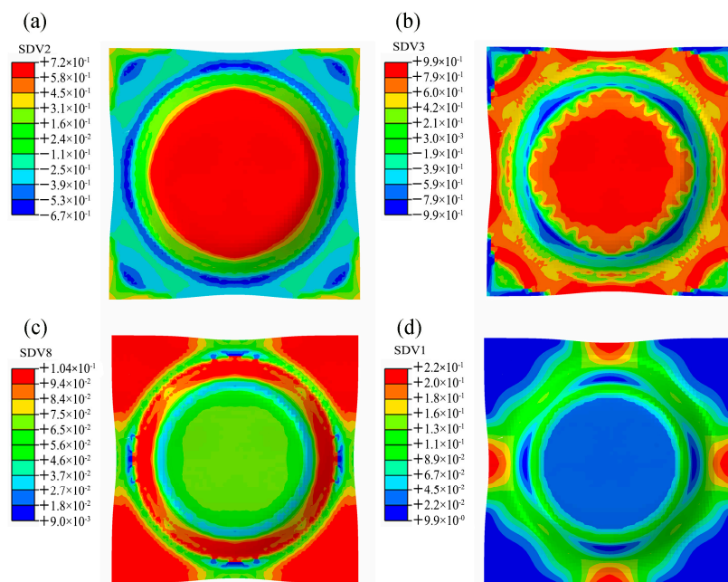
Figure 20. Marciniak simulation results when the stroke of the punch reaches 25 mm: (a) stress triaxiality; (b) Lode angle parameter; (c) retained austenite; (d) EPS.
