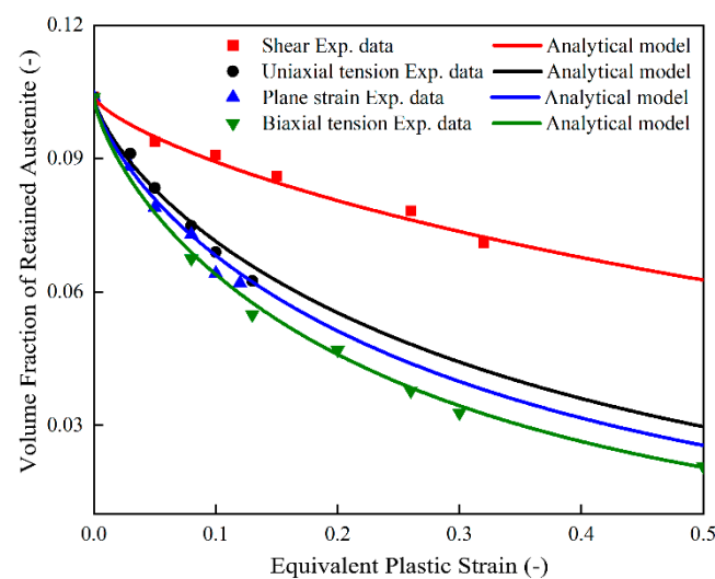
Figure 6. Comparisons of prediction results of austenite content evolution under different stress states.
