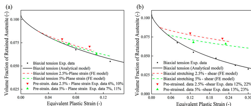
Figure 23. Distribution of retained austenite with varying EPS under different loading paths: (a) comparison of the experimental results of the VFRA test and the VFRA prediction results of the FE model under biaxial tension–plane strain tension at 6%, 10%, 7%, and 11% EPS; (b) comparison of the experimental results of the VFRA test and VFRA prediction results of the FE model under biaxial tension–pure shear at 12%, 22%, 13%, and 23% EPS.
