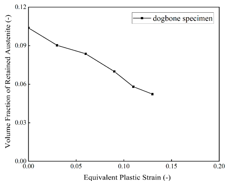
Figure 2. QP980 steel variation in retained austenite with EPS under uniaxial tension.
