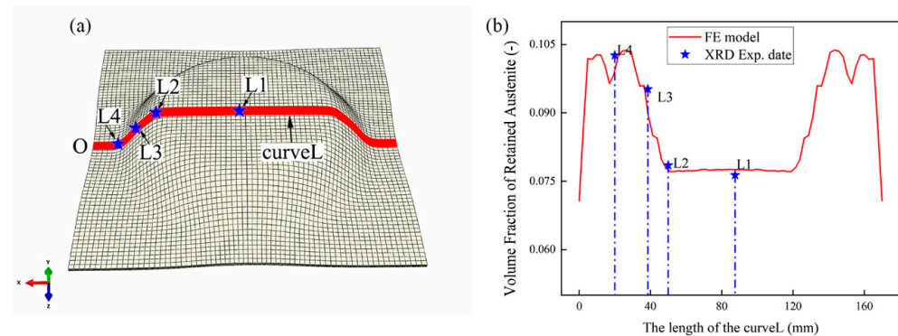
Figure 21. When the stroke of the punch reaches 25 mm, comparison between Marciniak test results and Prediction results of martensitic phase transformation by FE model: (a) schematic diagram of the location of XRD points; (b) the results of martensitic transformation predicted by FE model are compared with the experimental results.
