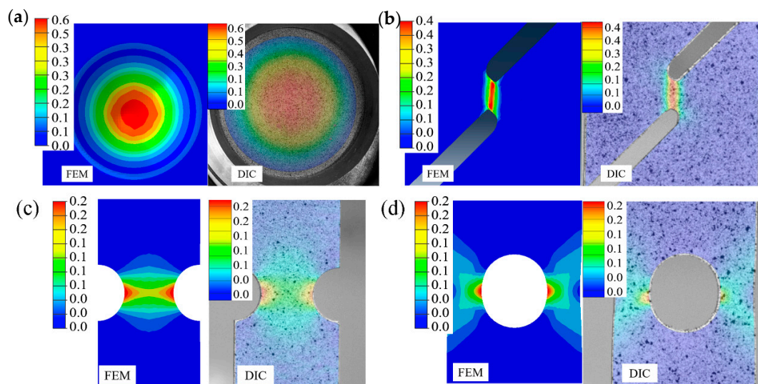
Figure 9. Comparison of strain distribution on a deformed surface in ARAMIS 2017 test (right) and FE model (left): (a) Nakajima specimen; (b) shear specimen; (c) notched specimen; (d) central hole specimen.
