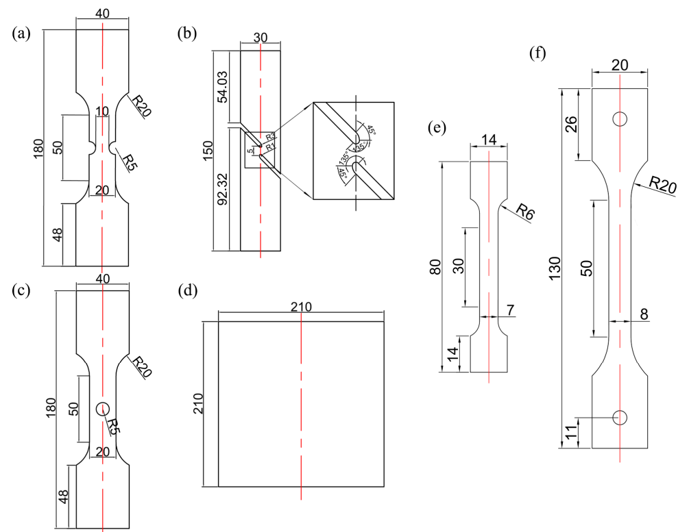
Figure 3. Shape and size of specimens: (a) notched; (b) shear; (c) central hole; (d) Nakajima specimen; (e) mini tensile specimen; (f) medium tensile specimen.
