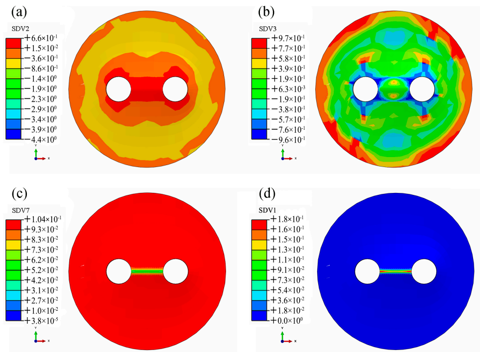
Figure 14. The FE simulated results of the two-hole specimen model after the second cyclic loading: (a) stress triaxiality; (b) Lode angle parameter; (c) retained austenite; (d) EPS.
