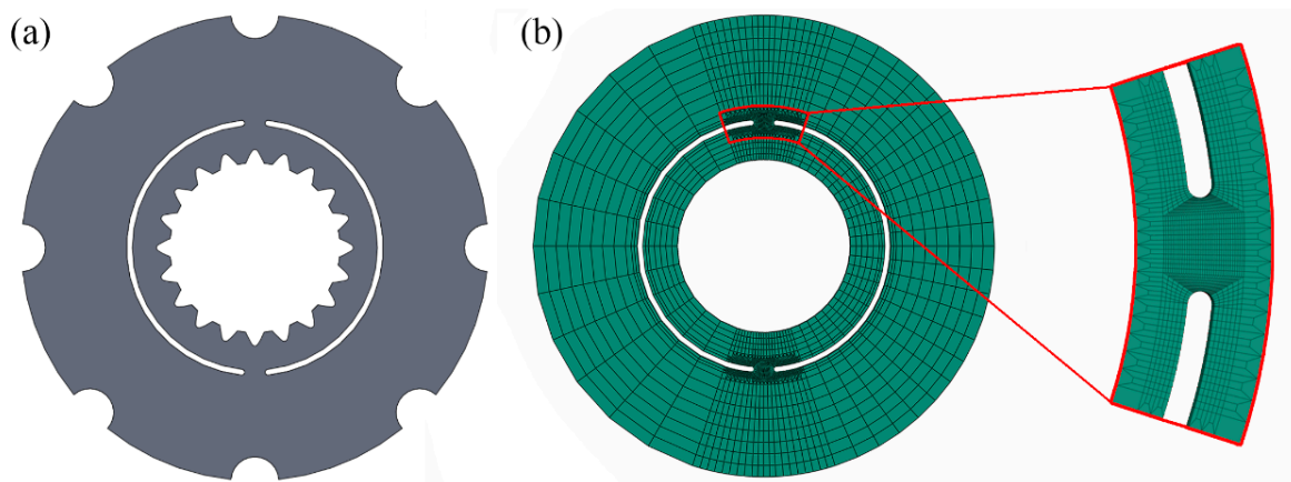
Figure 15. Schematic diagram of the twin bridge torsion shear specimen: (a) CAD model; (b) the simplified FE model.
