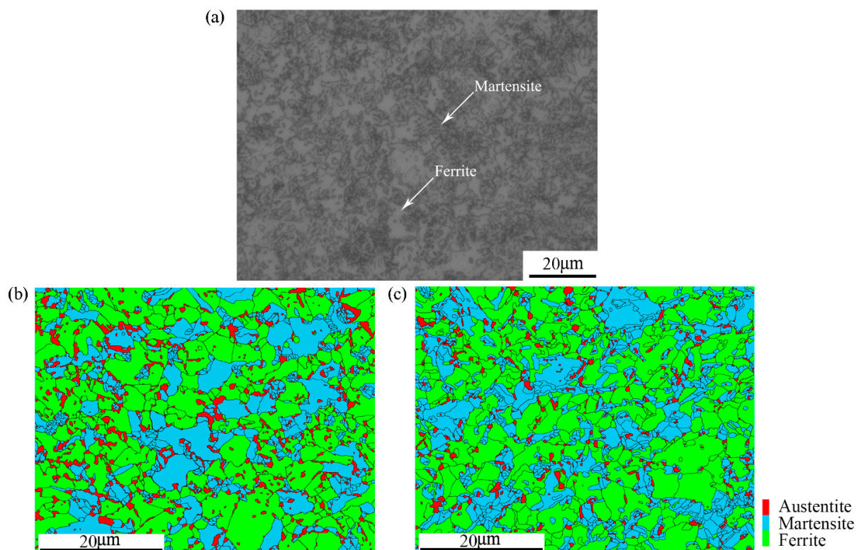
Figure 1. Microstructure of QP980 steel sheet: (a) martensite and ferrite are characterized by OM (1000×); (b) EBSD characterization of QP980 steel when \varepsilon_{eq} = 0 ; (c) EBSD characterization of QP980 steel when \varepsilon_{eq} = 0.11 .
