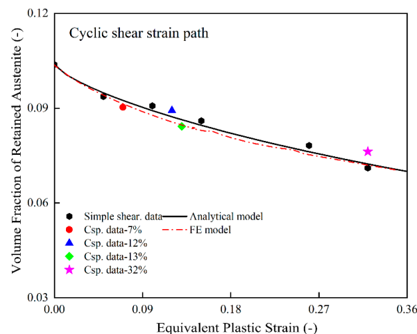
Figure 17. Evolution of retained austenite with EPS during cyclic shear strain loading: these include experimental results from tests of retained austenite volume fractions at EPS of 7%, 12%, 13%, and 32%, and predictions of VFRA from analytical model and FE model.
