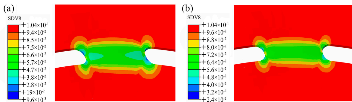
Figure 18. Distribution of retained austenite at different torsion stages in the critical area of the twin bridge torsion shear specimen: (a) \varepsilon_{eq} = 0.07 ; (b) \varepsilon_{eq} = 0.12 .
