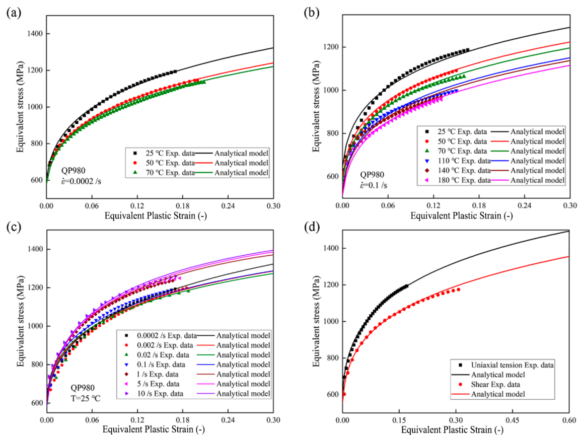
Figure 7. Analytical predictions and experimental data of equivalent stress-strain curves at various strain rates and temperature: (a) equivalent stress-strain curves at various temperature and a fixed quasi-static strain rates ( \dot{\varepsilon} = 0.0002/s ); (b) equivalent stress-strain curves at various temperature and a fixed medium strain rates ( \dot{\varepsilon} = 0.1/s ); (c) equivalent stress-strain curves at various strain rate and a fixed temperature ( T = 25\text{ }^{\circ}\text{C} ); (d) equivalent stress-strain curves under tension and shear stress conditions.
