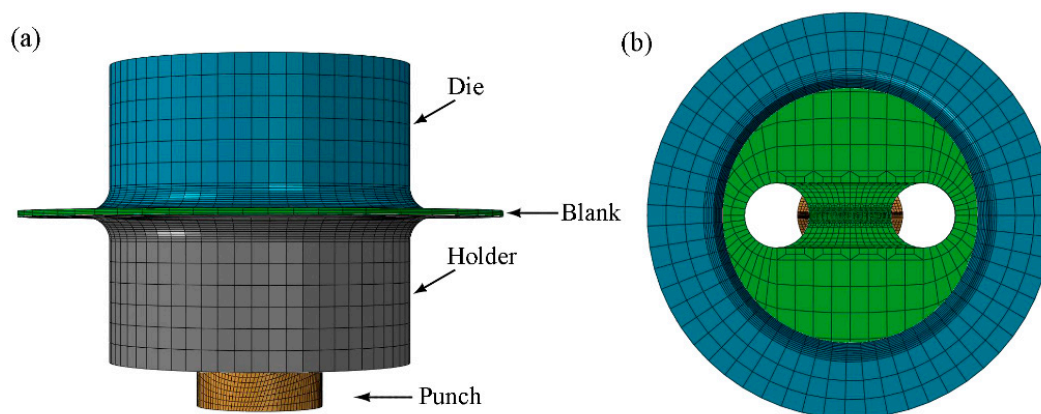
Figure 11. The FE model of the cyclic plane strain path loading: (a) front view; (b) vertical view.
