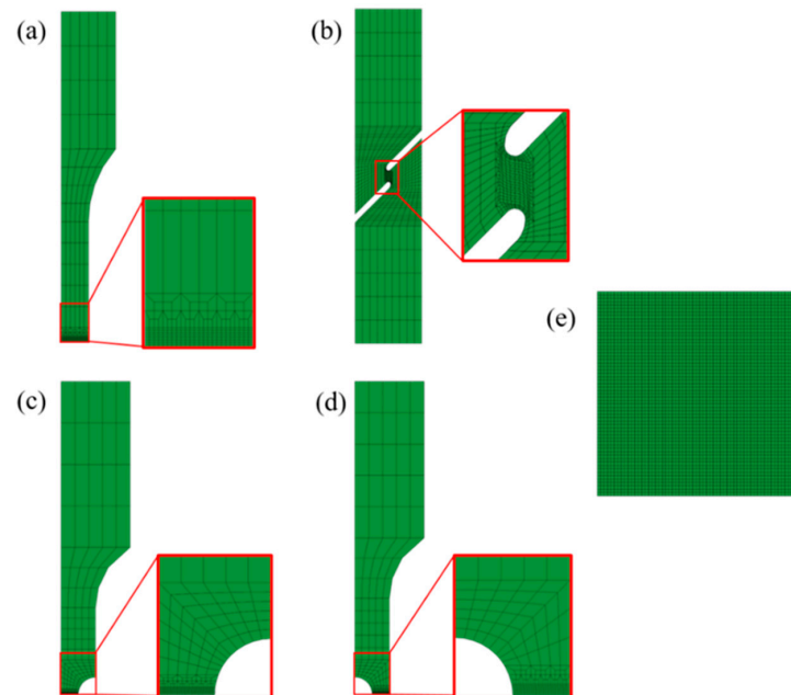
Figure 8. Meshes at ambient temperature for specimens under various stress mode: (a) Dog-bone specimen; (b) shear specimen; (c) notched specimen; (d) central hole specimen; (e) Nakajima specimen.
