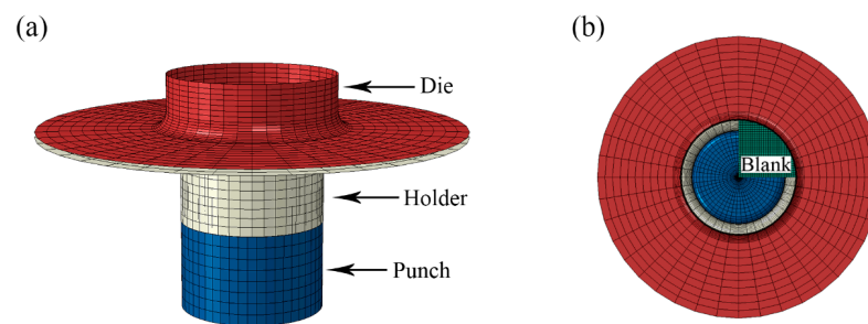
Figure 19. Marciniak test FE model: (a) front view; (b) vertical view.
