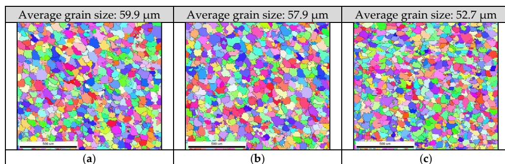
Figure 14. EBSD results for (a) one, (b) three, and (c) five repetitions. The specimens were prepared at a welding speed of 0.5 m/min and R_{EN} of 0.5. Scale bar = 500 \mu\text{m} .
