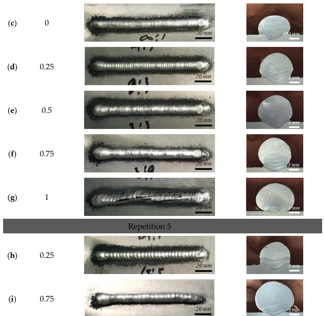
Figure 10. Bead appearance and cross-sectional images depending on R_{EN} and repetition conditions. Specimens were fabricated at a welding speed of 0.5 m/min.
