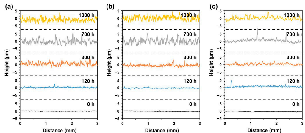
Figure 7. Representative surface topographic profiles of the oxide scales, obtained from contact profilometer, formed on the (a) SS301, (b) DS2205 and (c) DS2507 after exposing to molten salts for different times.
