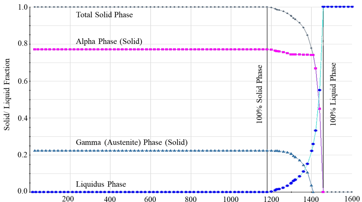
Figure 5. The fraction of liquid and solid phase vs. temperature for 17-4 PH.
