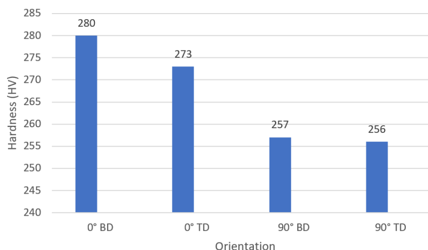
Figure 12. Hardness value for 0^\circ and 90^\circ build direction.
