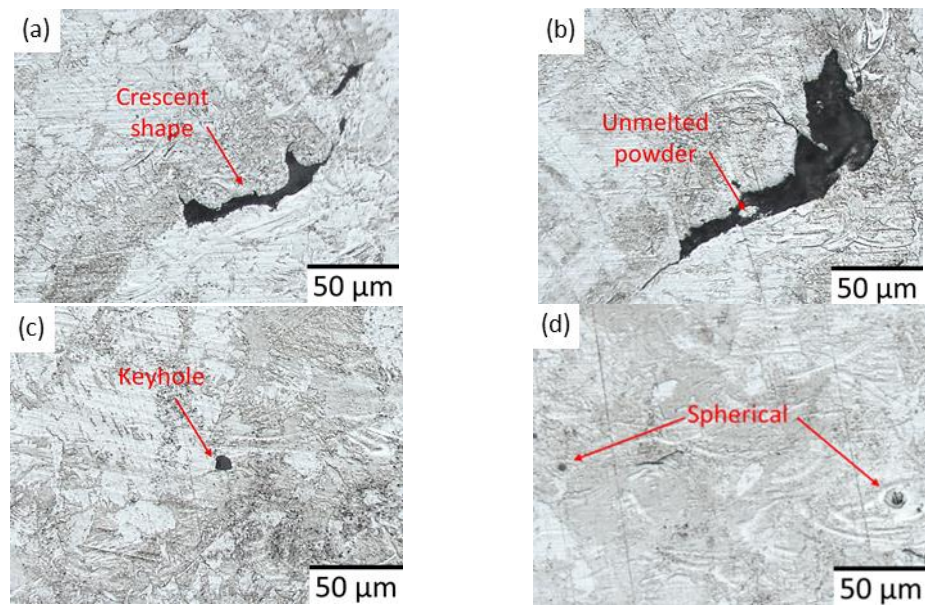
Figure 14. The types of porosity observed from three different areas of 45° build direction; (a) crescent shape, (b) unmelted powder, (c) keyhole and (d) spherical porosity.
