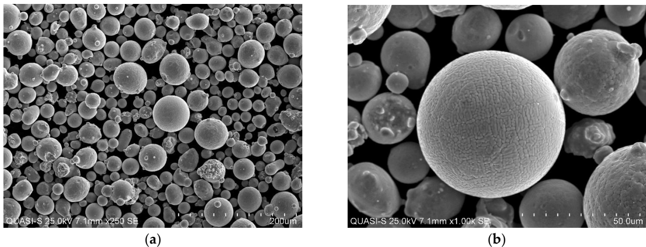
Figure 3. Powder morphology reveal by SEM observation at (a) 250 and (b) 1000 magnification scale.
