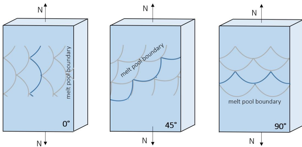
Figure 18. The direction of the melt pool boundary for each build direction relative to the load direction.
