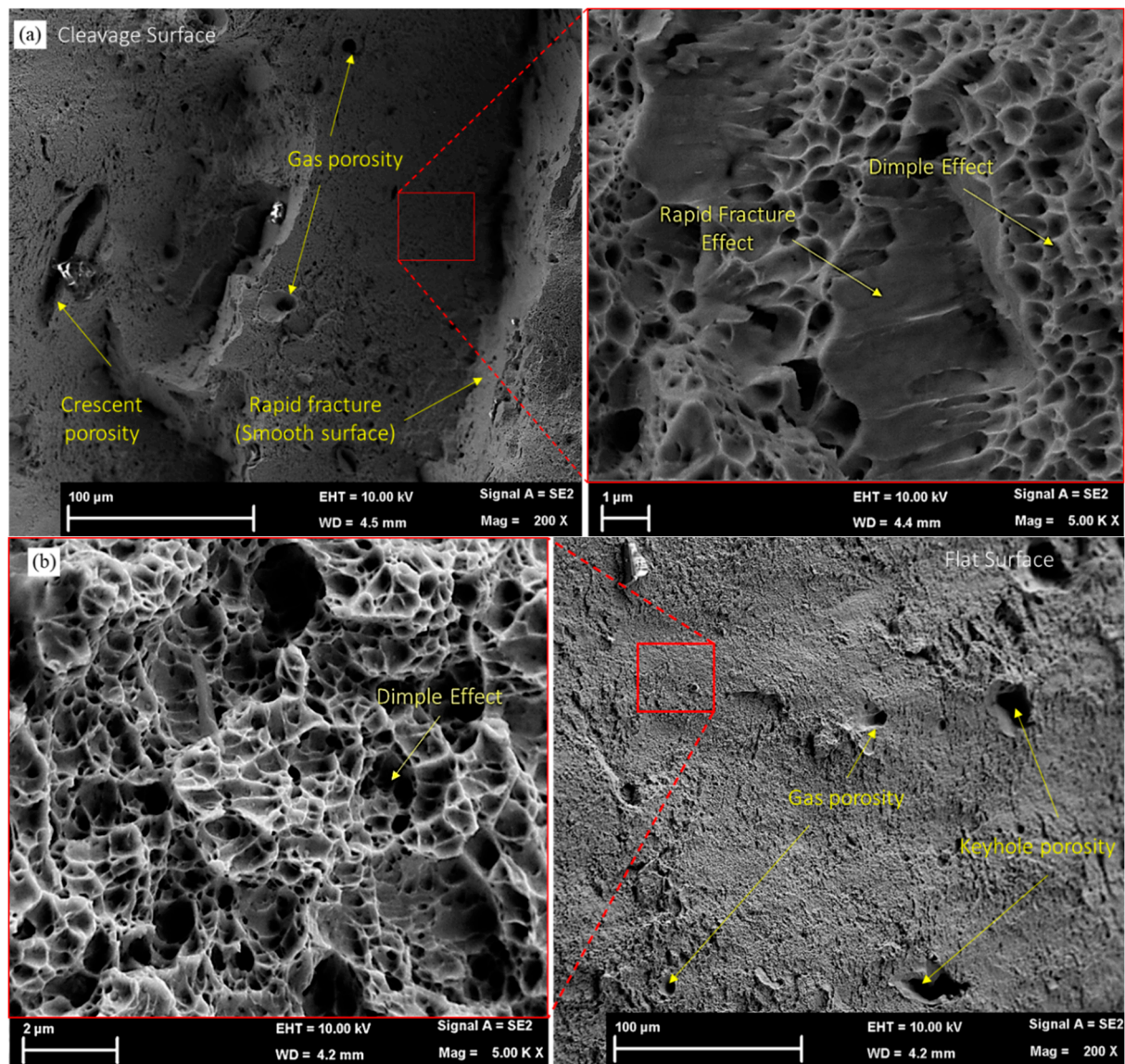
Figure 21. SEM of a fractured surface under 200 \times and 5000 \times magnification for (a) cleavage surface and (b) flat surface.
