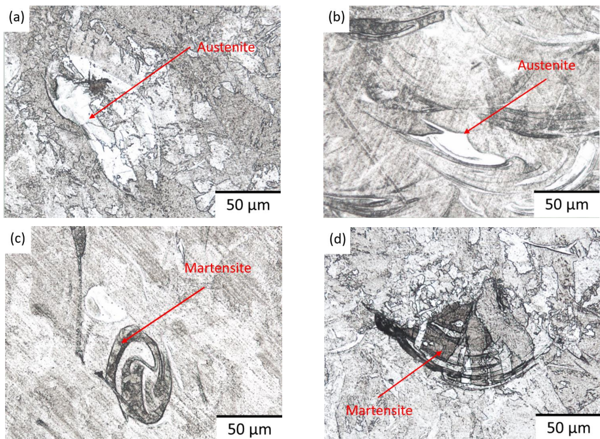
Figure 11. Identification of (a,b) austenite phase in build direction and transverse direction and (c,d) martensite phase in build and transverse direction.
