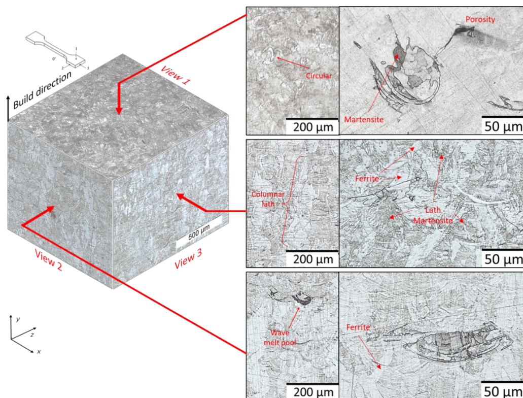
Figure 7. Microstructure profile for 0^\circ build direction.
