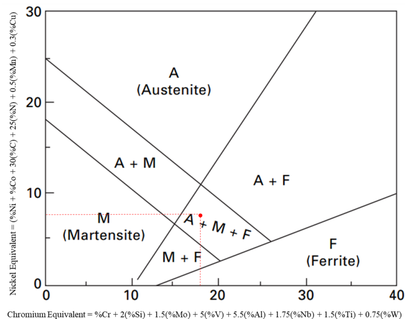
Figure 1. Possible phases of 17-4 PH shown in red dot according to Schaeffler Diagram (reproduced with permission from Elsevier, 2022) [15,16].
