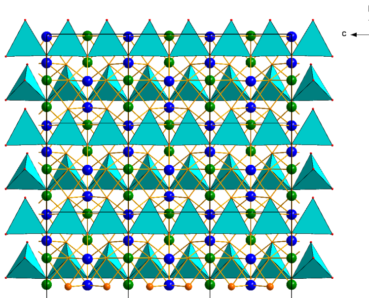
Figure 10. The crystal structure of cerromojonite projected down [100] (six unit-cells). Symbols as in Figure 9. \text{CuSe}_4 tetrahedra are depicted as light blue polyhedra. The unit-cell and orientation of the figure are outlined.
