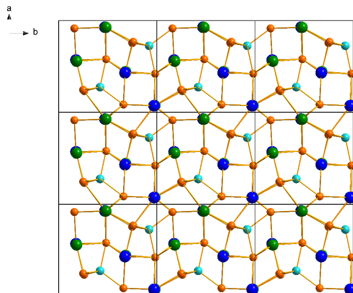
Figure 9. The crystal structure of cerromojonite projected down [001] (six unit-cells). The unit-cell and orientation of the figure are outlined. Symbols: Bi = green dots, Pb = blue dots, Cu = light blue dots, Se = orange dots.
