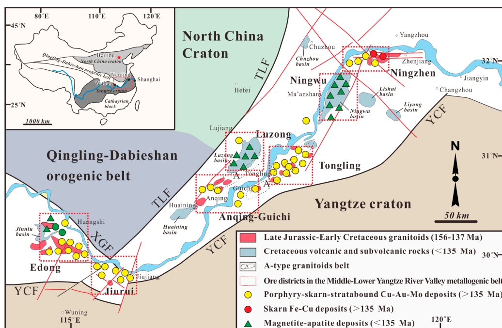
Figure 1. Location of the Tongling ore district in the Middle–Lower Yangtze River Valley metallogenic belt (after [26]). TLF: Tancheng–Luijiang fault; XGF: Xiangfan–Guangji fault; YCF: Yangxing–Changzhou fault.
