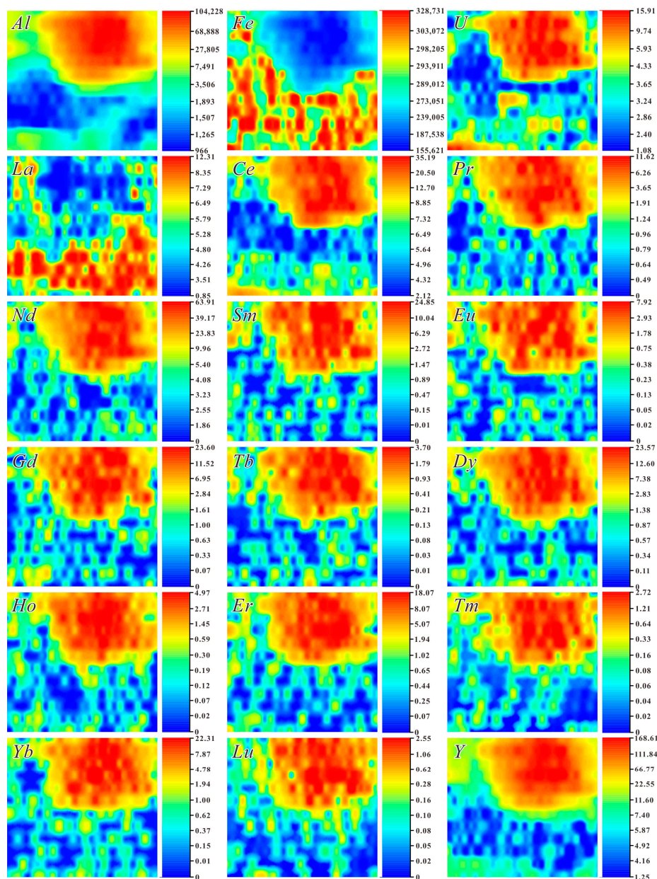
Figure 5. LA-ICP-MS trace element maps of the Xinqiao garnet; all maps show ppm abundances on a log scale.
