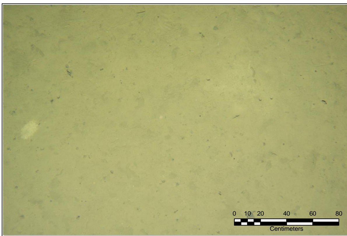
Figure 11. Sediment drift example photo. Source: TOML image 2015_08_10_225306.
