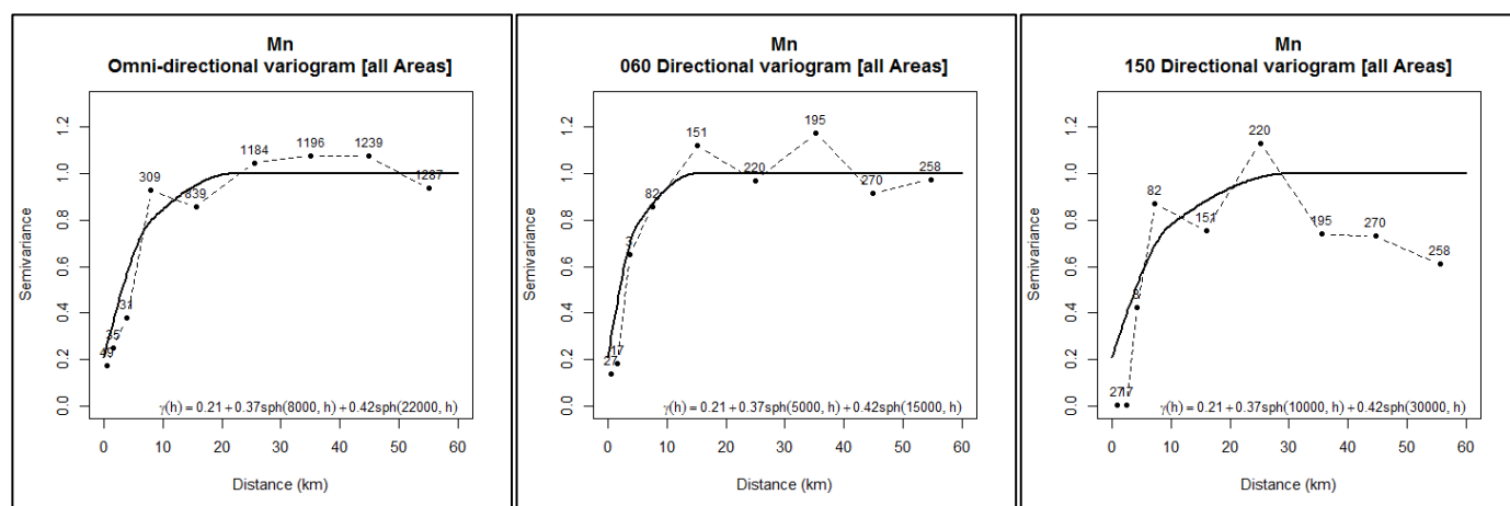
Figure 26. Mn omni-directional, 060° and 150° directional variograms. Source: [12].
