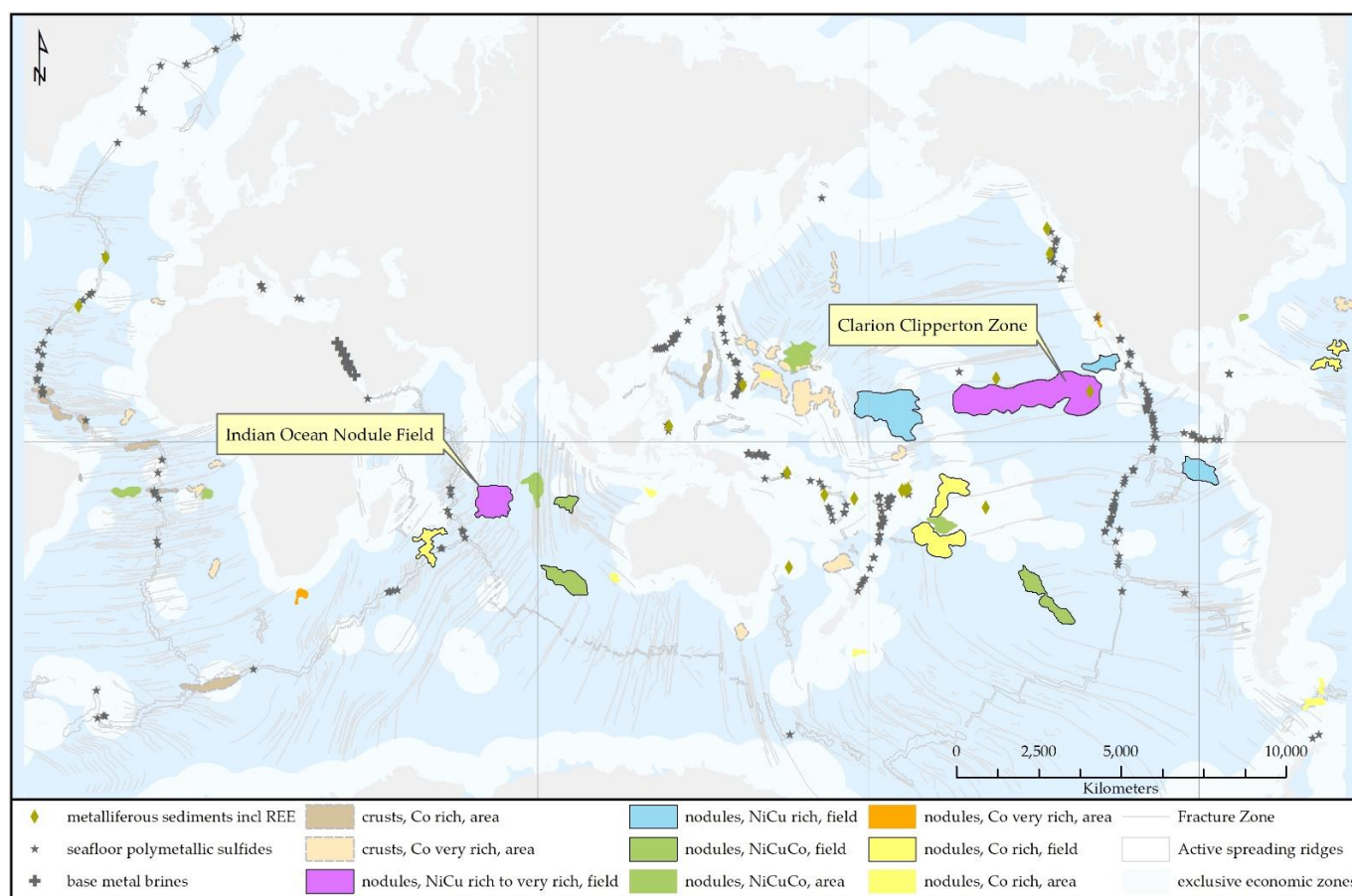
Figure 1. Locations of the Clarion Clipperton Zone and Indian Ocean Nodule Field. Adapted from Andreev et al. [6] and Matthews et al. [7]. Rich Co is generally >0.4\% , very rich Co is >0.8\% , NiCuCo is 0.7\text{--}1.7\% Ni + Cu, rich Ni-Cu is >1.7\% Ni + Cu, and very rich Ni-Cu is >2.5\% Ni + Cu; the fields are better constrained from sampling than the areas.
