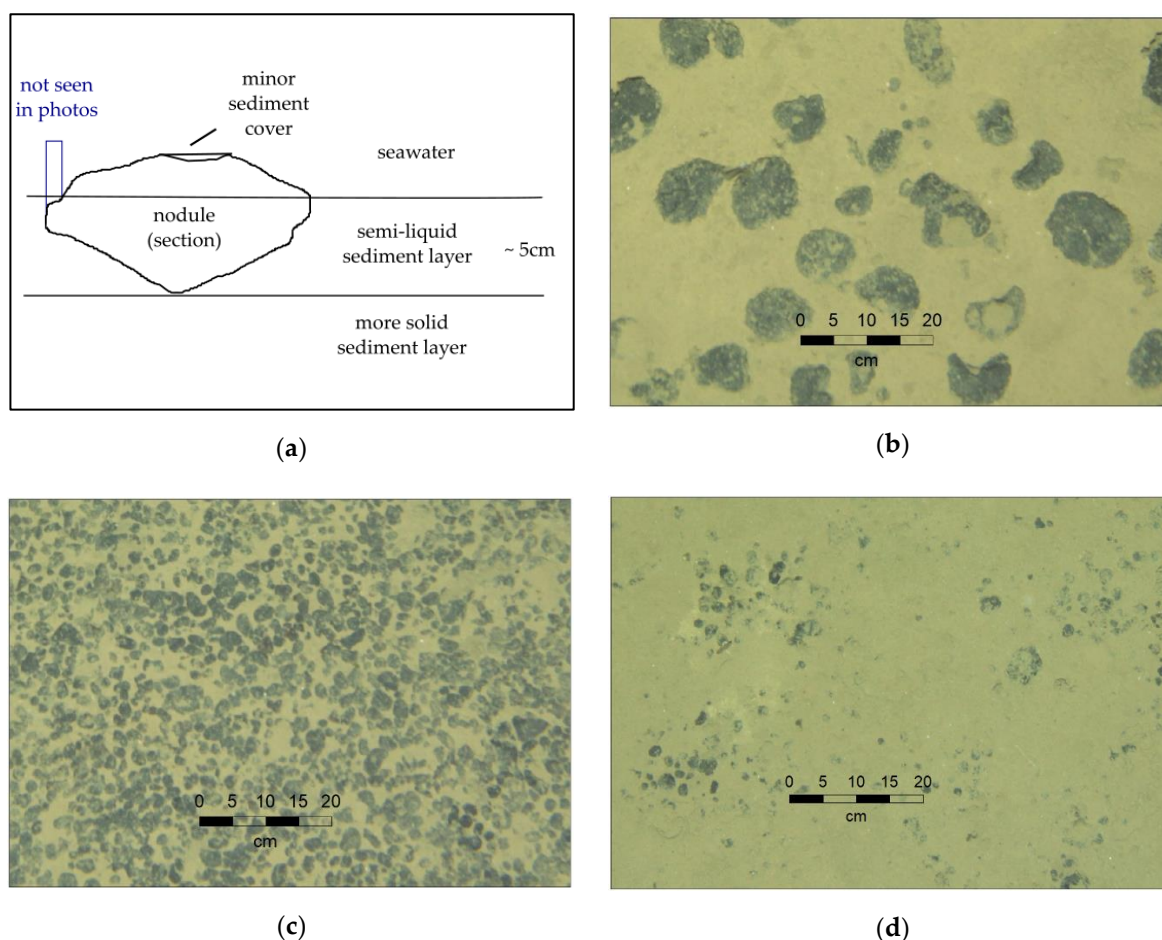
Figure 5. Polymetallic nodules on the seabed. (a) Schematic cross-section of nodules on the seabed; (b) example of large nodules (source: Tonga Offshore Mining Limited (TOML) image 2015_08_17_044250); (c) example of small nodules (source: TOML image 2015_08_17_105534); (d) example of covered nodules (source: TOML image 2015_09_16_183847).
