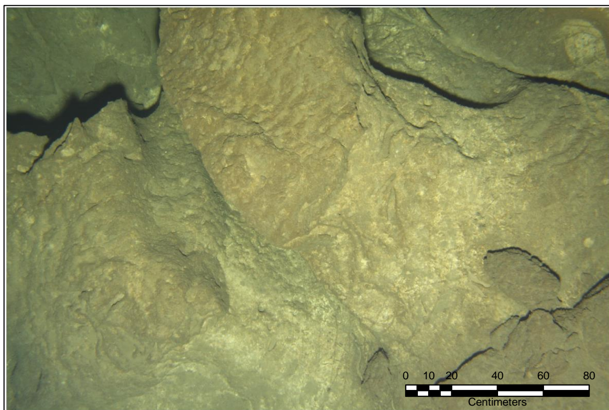
Figure 13. Chalk escarpment example photo. Source: TOML image 2015_08_10_205331.
