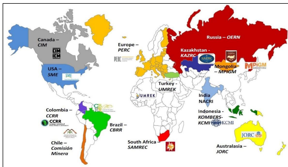
Figure 3. Map of member coders Committee for Mineral Reserves International Reporting Standards (as of August 2019). Source: Committee for Mineral Reserves International Reporting Standards [16].
