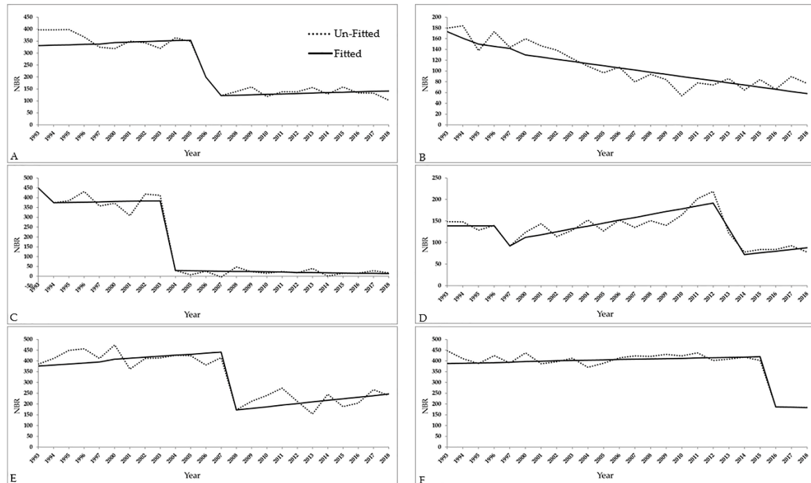
Figure S1. Examples of temporal change trajectories: A: Plantation changed to urban, B: Home garden changed to peri-urban and subsequently to urban, C: Forest changed to water, D: Peri-urban changed to urban, E: Rice paddy changed to water, F: Forest changed to urban.
