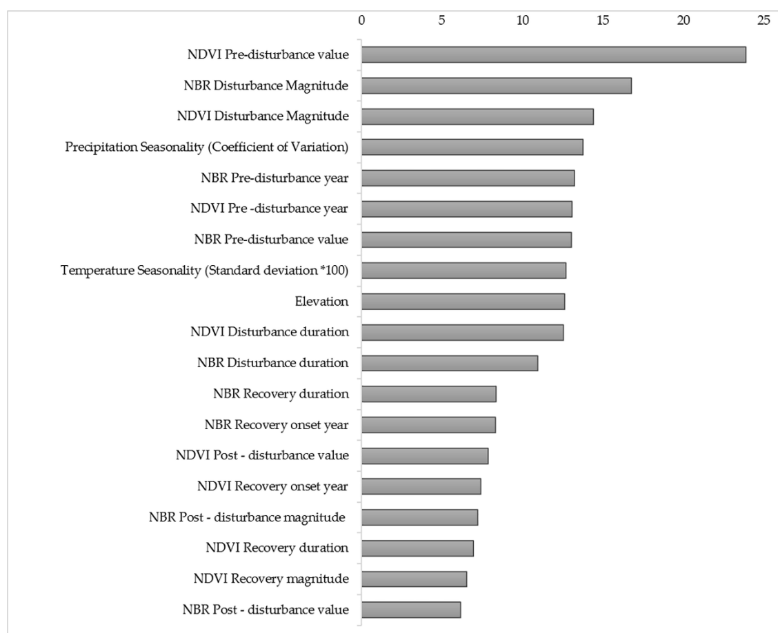
Figure S2. Variable importance graph prepared based on mean decrease accuracy of the random forest model.
