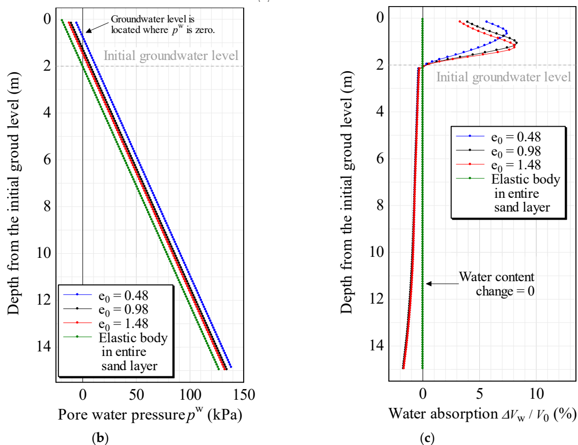
Figure 14. Distributions of degree of saturation, pore water pressure, and the amount of water absorption when the void ratio of the unsaturated sand layer modeled as an elastic body varies: (a) degree of saturation; (b) pore water pressure; and (c) amount of water absorption.
