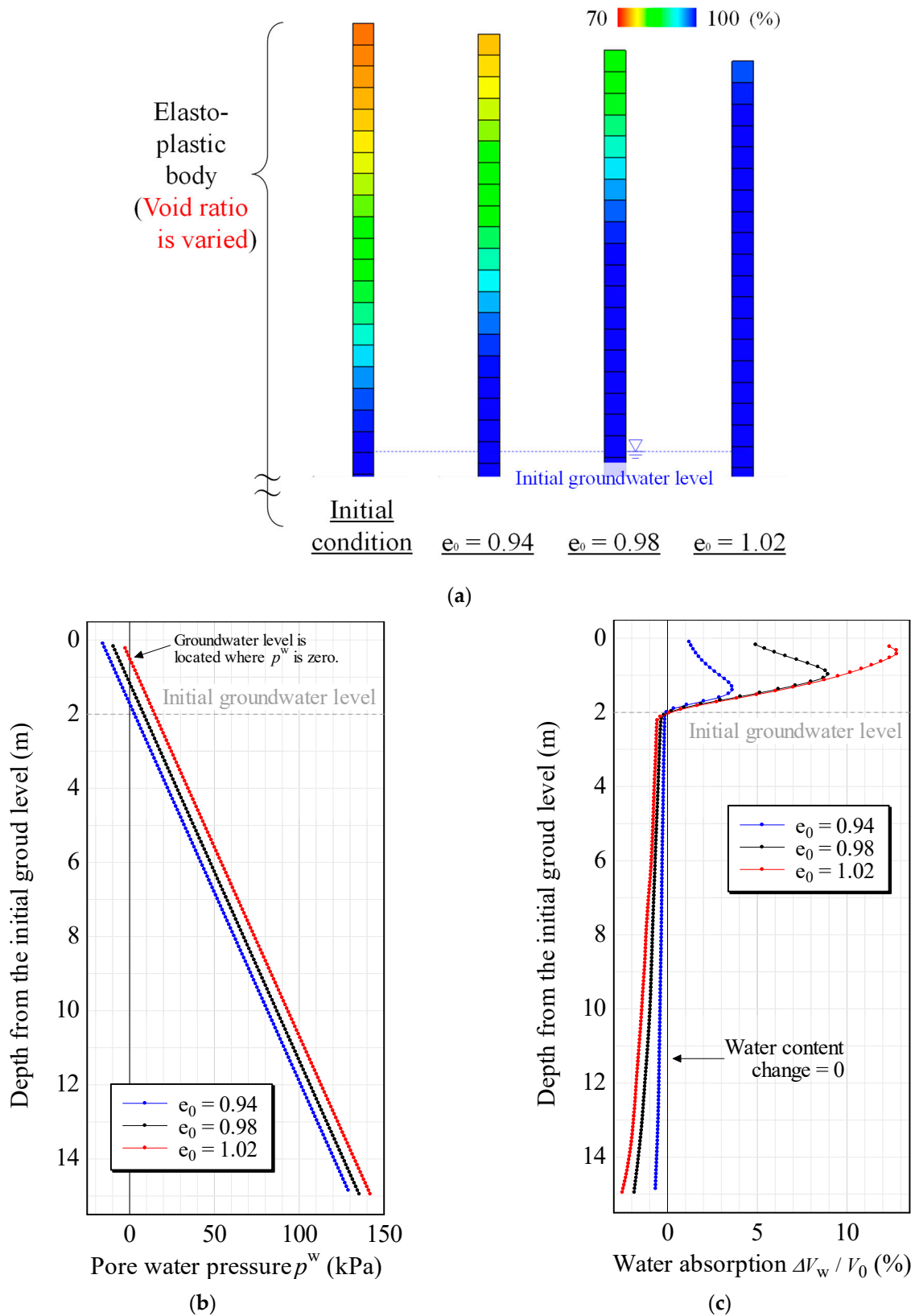
Figure 13. Distributions of degree of saturation, pore water pressure, and the amount of water absorption when the void ratio of the entire sand layer varies: (a) degree of saturation; (b) pore water pressure; and (c) amount of water absorption.
