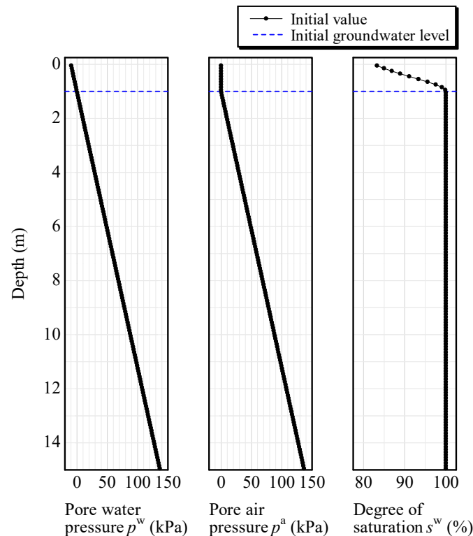
Figure 4. Initial values for pore water/air pressure and degree of saturation in the sand layer.
