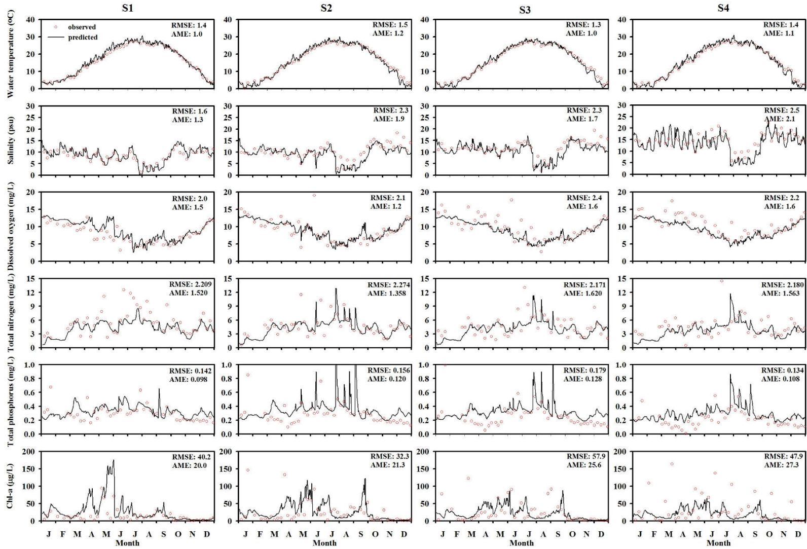
Figure S1. Comparisons of predicted and observed water quality constituents in the surface layer.
