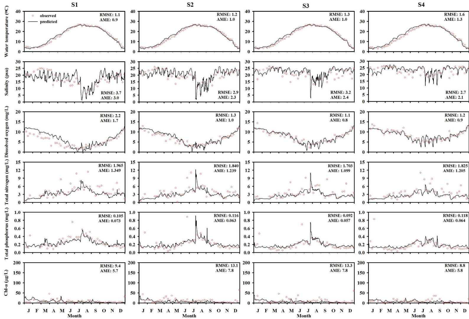
Figure S2. Comparisons of predicted and observed water quality constituents in the bottom layer.
