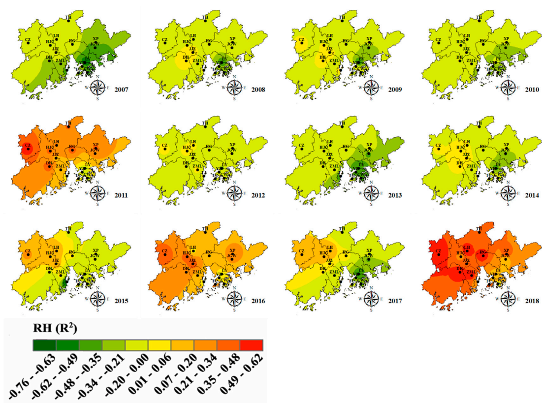
Figure S3. Annual coefficients of determination ( R^2 ) between the baseline of daily MDA8 and RH.
