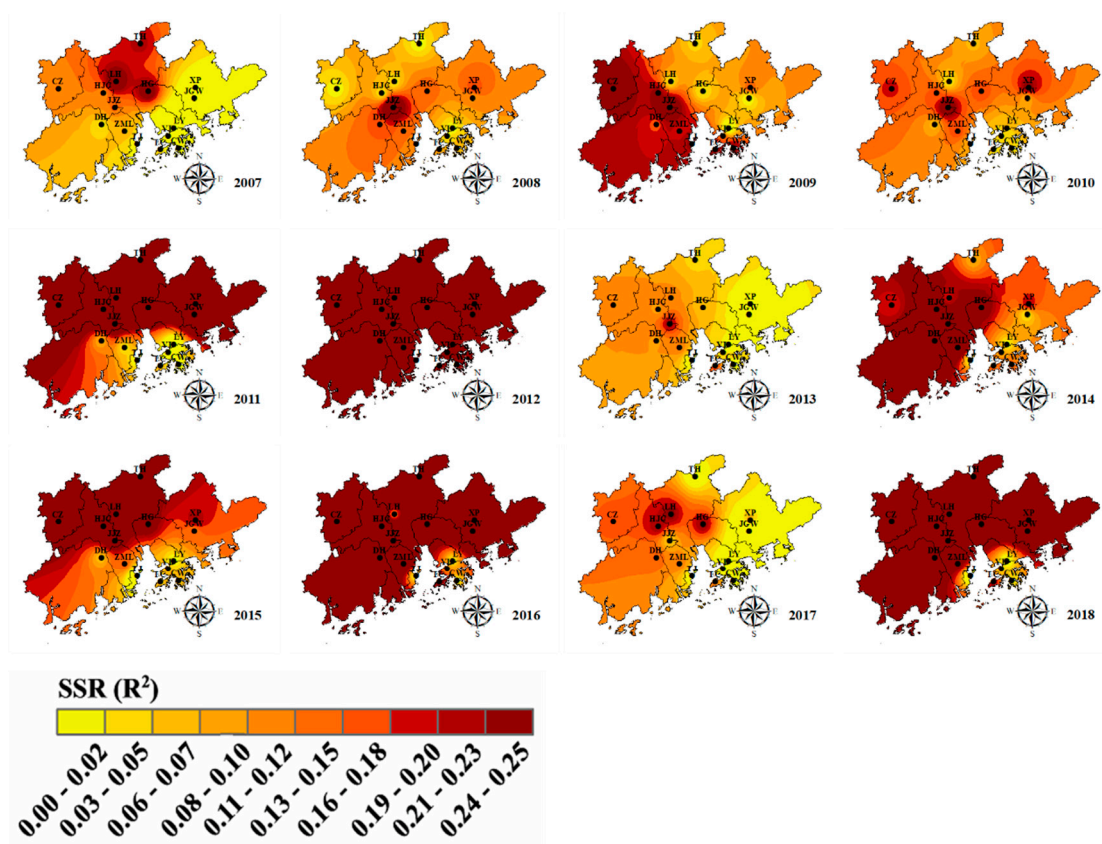
Figure S1. Annual coefficients of determination ( R^2 ) between the baseline of daily MDA8 and SSR.
