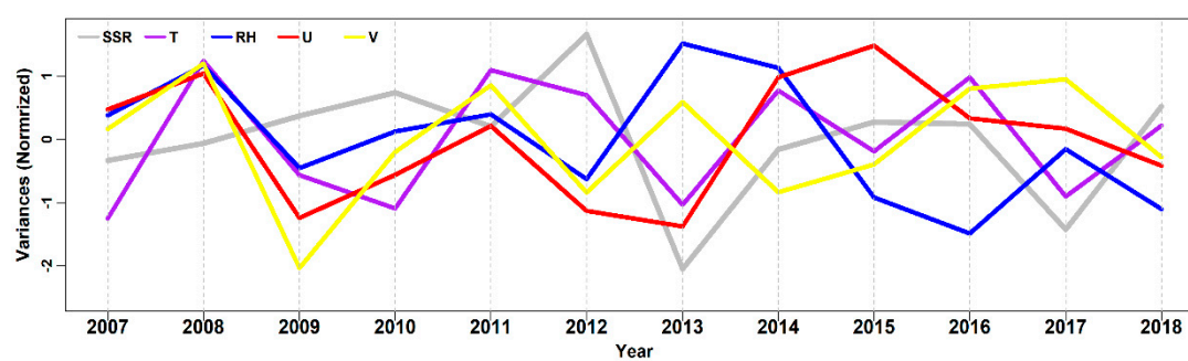
Figure S6. Annual variances of each meteorological variable.
