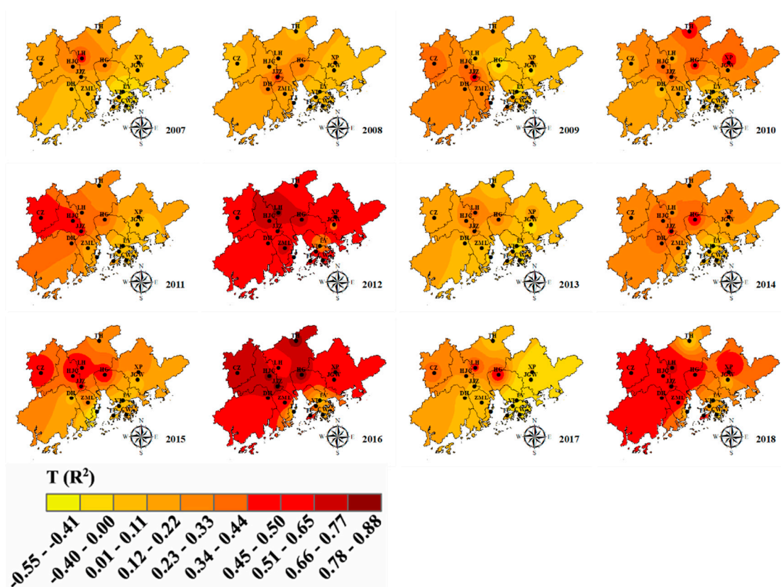
Figure S2. Annual coefficients of determination ( R^2 ) between the baseline of daily MDA8 and T.
