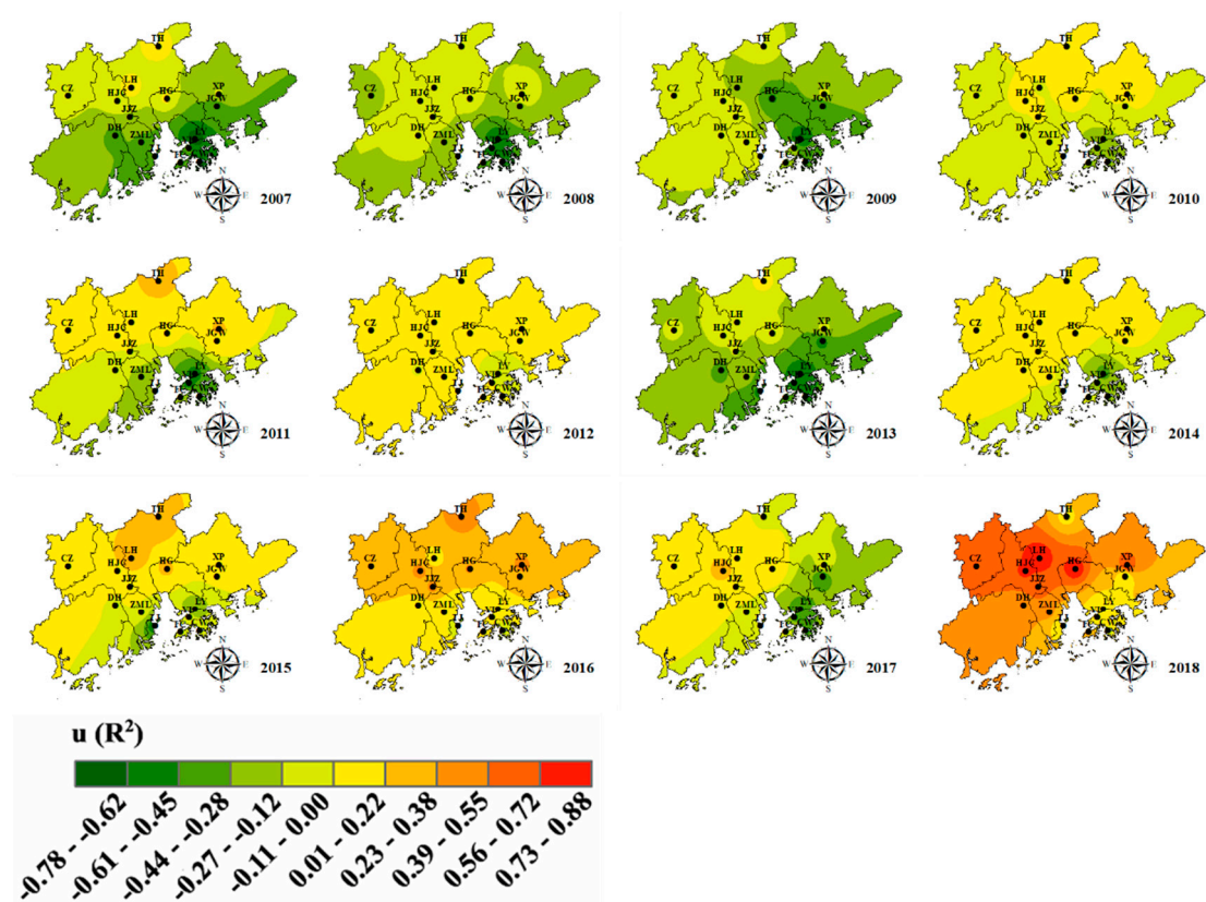
Figure S4. Annual coefficients of determination ( R^2 ) between the baseline of daily MDA8 and u .
