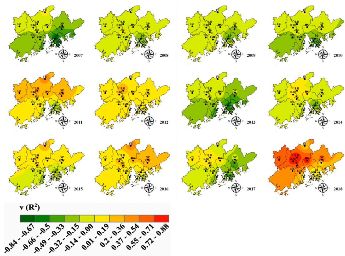
Figure S5. Annual coefficients of determination ( R^2 ) between the baseline of daily MDA8 and v .
