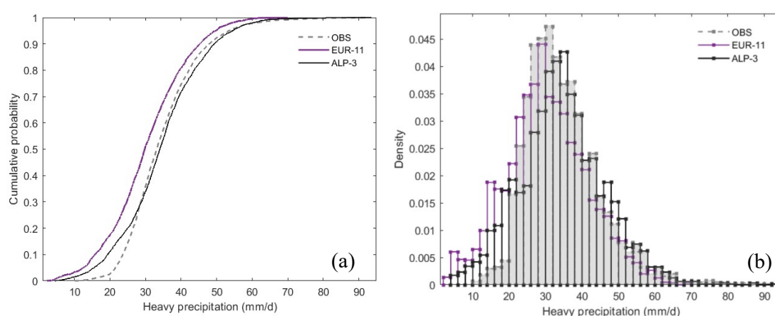
Figure 3. Empirical cumulative distribution functions (a) and probability density functions (b) related to heavy precipitation 99p from daily data. The observations are filled with a grey area.
