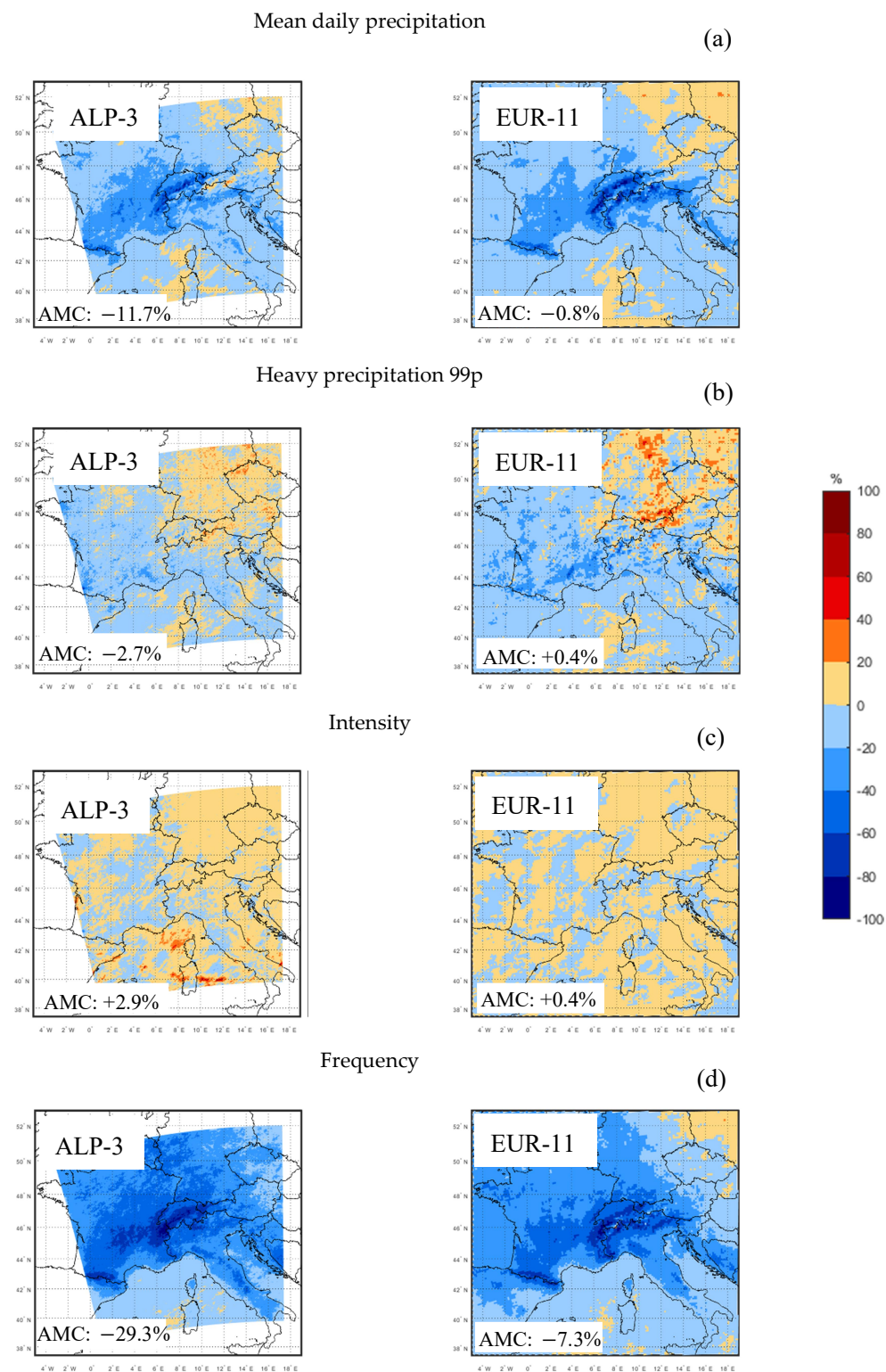
Figure 6. Changes in daily mean precipitation (a), heavy precipitation (b), intensity (c) and frequency (d) related to summer season (JJA) projected at the end of century (2090–2099) with respect to the historical period (1996–2005).
