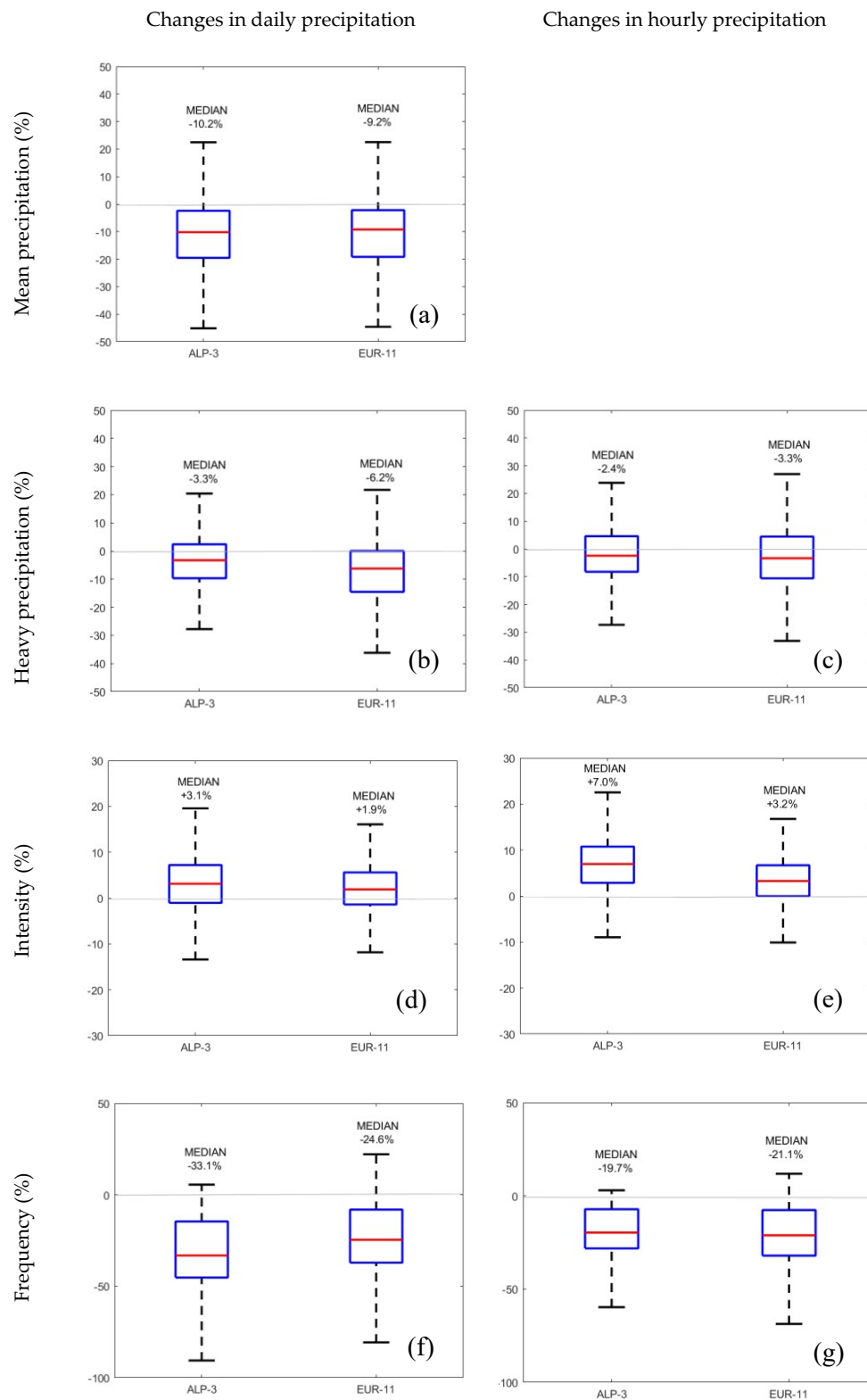
Figure 8. “Whiskers” box plots of daily (a,b,d,f) and hourly (c,e,g) projected changes of precipitation resulting from ALP-3 and EUR-11 simulations.
