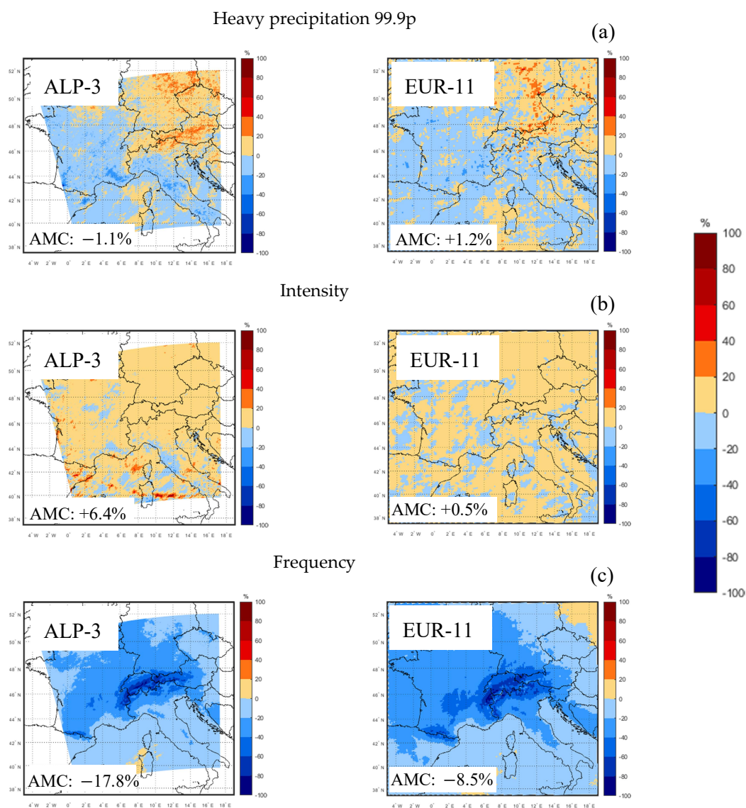
Figure 7. Changes in hourly heavy precipitation (a), intensity (b) and frequency (c) related to summer season (JJA) projected at the end of century (2090–2099) with respect to the historical period (1996–2005).
