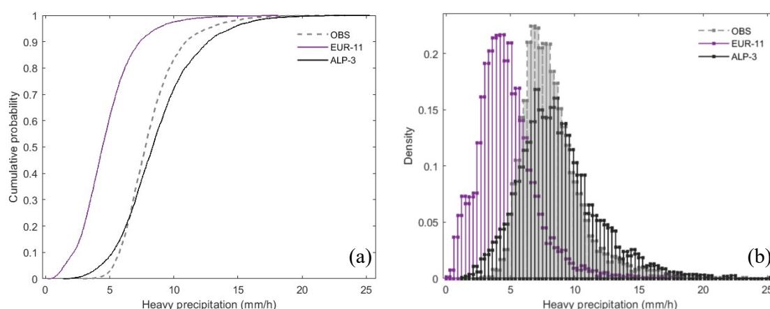
Figure 5. The empirical cumulative distribution functions (a) and probability density functions, (b) related to heavy precipitation 99.9p from hourly data. The observations are filled with a grey area.
