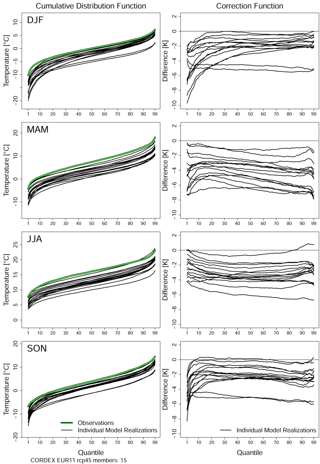
Figure S1 Cumulative distributions of daily mean temperature (left) and correction functions (right) for 15 climate models' simulations – an example for the low concentration RCP4.5 scenario
