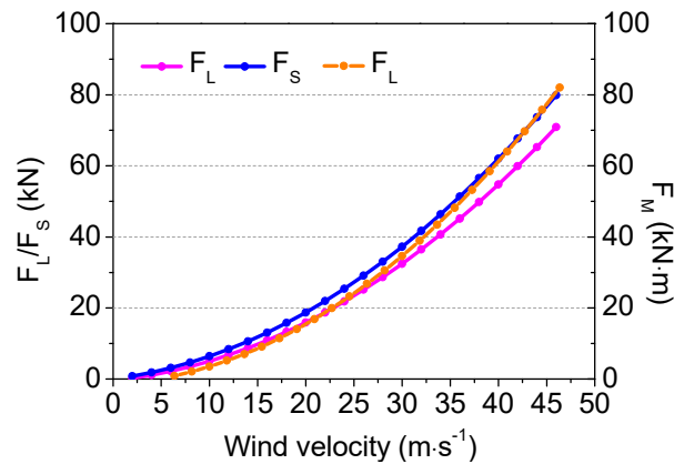
Figure 10. As in Figure 9 but the impact of wind velocity variations assuming an easterly wind (90°).
