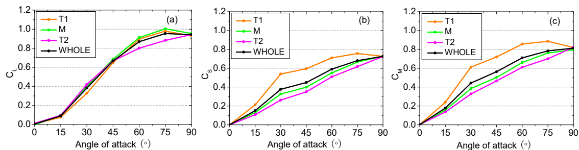
Figure 8. Aerodynamic force coefficients of rail vehicles versus angle of attack derived from Equation (9).
