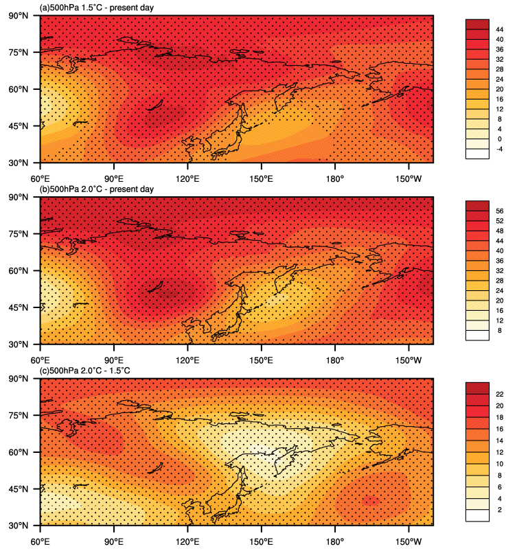
Figure S1. Regional mean changes in 500 hPa geopotential height in (a) 1.5 °C warming relative to the present day, (b) 2.0 °C warming relative to the present day, and (c) 2.0 °C warming relative to 1.5 °C warming. The dotted areas are statistically significant at the 5% level according to the Student's t -test.
