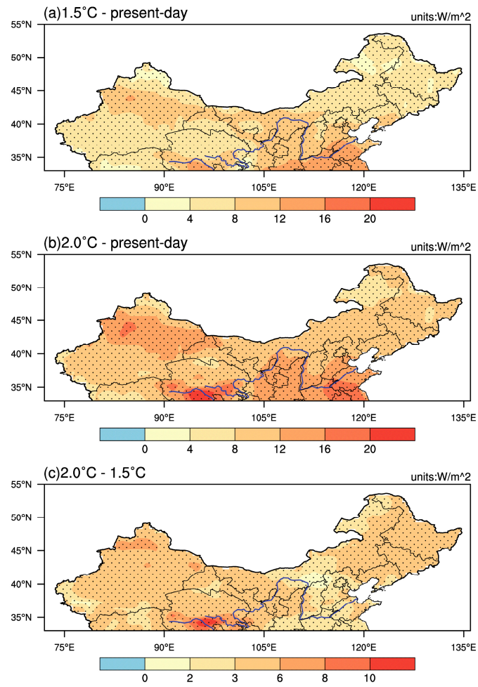
Figure S2. Regional mean changes in surface net radiation flux in (a) 1.5 °C warming relative to the present day, (b) 2.0 °C warming relative to the present day, and (c) 2.0 °C warming relative to 1.5 °C warming. The dotted areas are statistically significant at the 5% level according to the Student's t -test.
