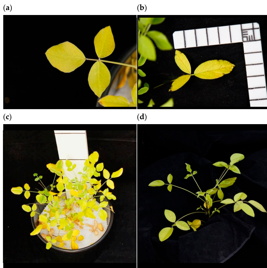
Figure 10. Leaf and whole plant symptoms of Lanza ® tedera (a,c) and Palma (b,d) grown in soils with very low sulphur ( <2 \text{ mg kg}^{-1} ). Photos were taken at 12 weeks old, except panel (d), taken at 8 weeks old.
