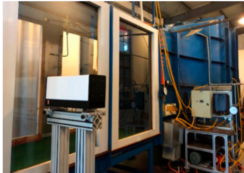
Figure 3. Atomization characteristics test device. 1—pump, 2—medicine box, 3—wind tunnel, 4—DP-02 laser particle size analyzer, 5—pressure regulating valve, 6—pressure gauge, 7—lifting guide rail, 8—spout, and 9—nozzle.
