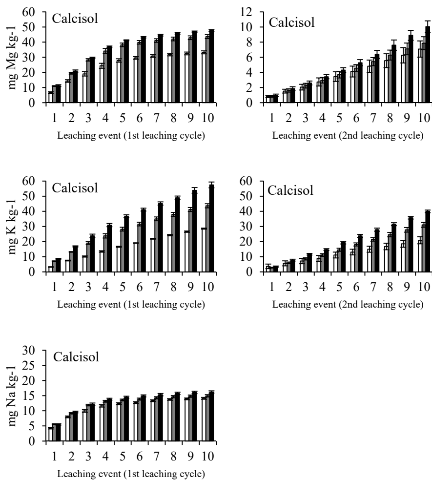
Figure S1: Cumulative leaching losses of Ca, Mg, K and Na from Acrisol and Calcisol. Bars indicate standard error of the mean (n=4).
