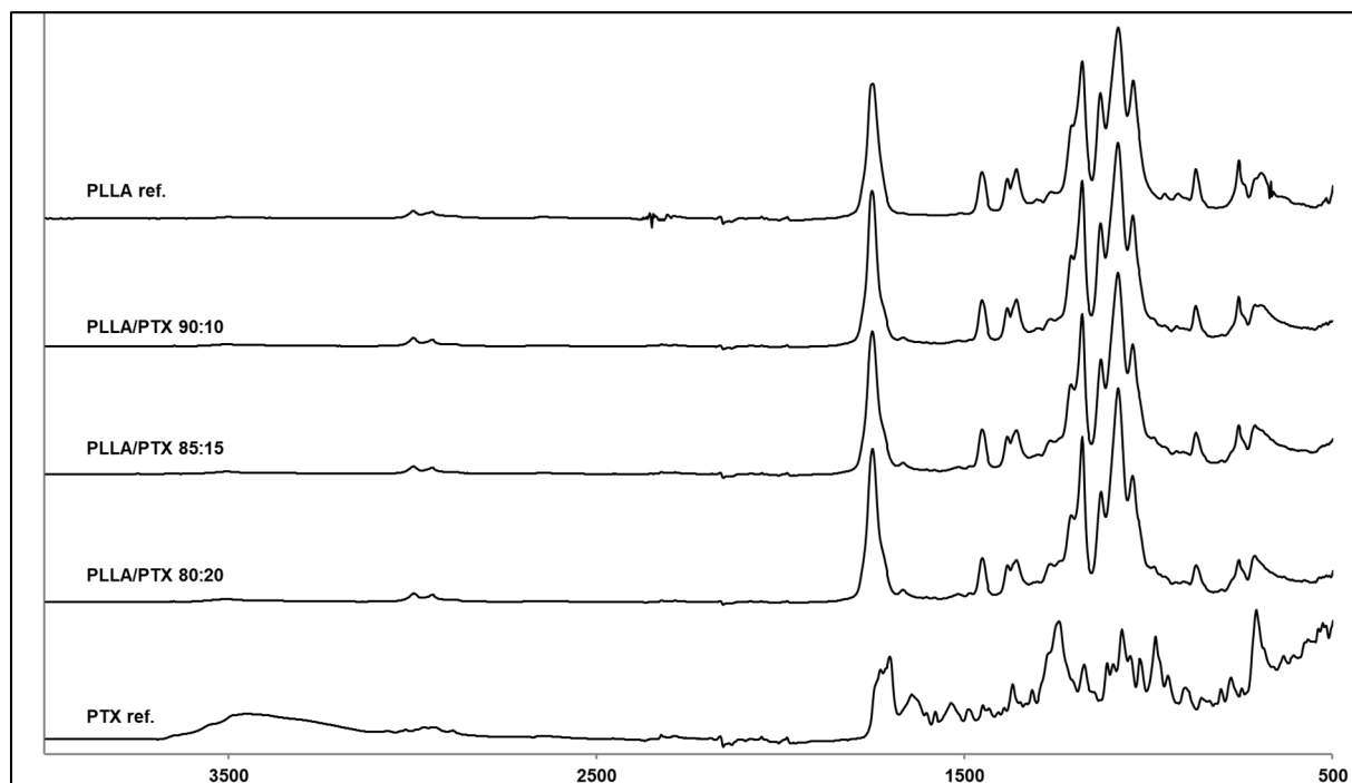
Figure S2.2: IR spectra of PLLA and PLLA with incorporated paclitaxel at 10, 15 and 20 w/w% and paclitaxel reference spectrum.
