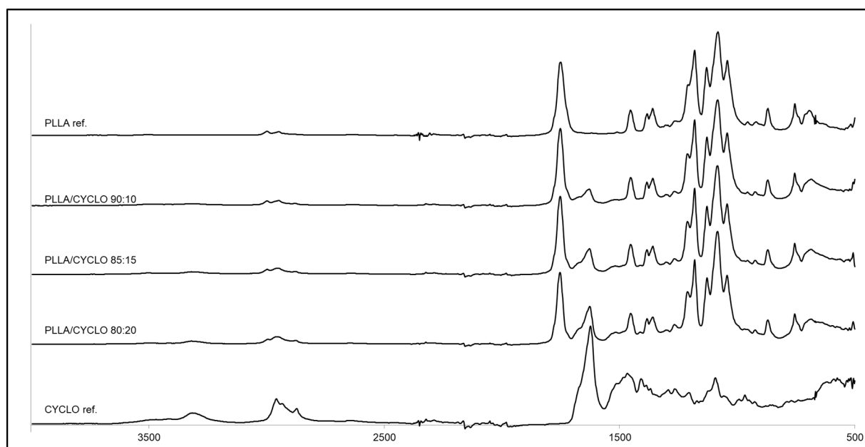
Figure S2.4: IR spectra of PLLA and PLLA with incorporated cyclosporine A at 10, 15 and 20 w/w% and cyclosporine A reference spectrum.
