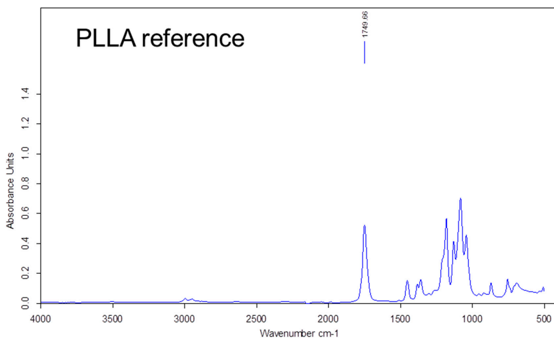
Figure S2: IR spectra of PLLA and PLLA with incorporated cyclosporine A at a ratio of CYCLO/PLLA = 10/90 w/w% with assigned bands for determination of drug incorporation.
