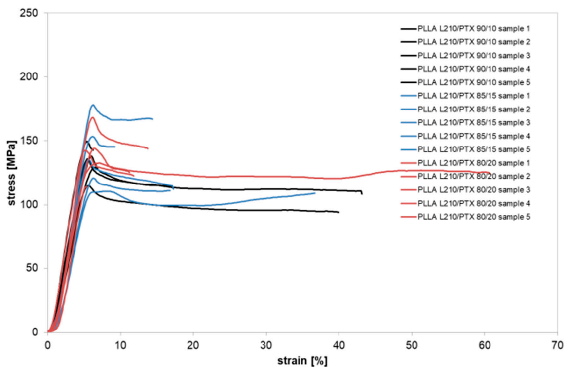
Figure S7.2: Stress strain curves of spray-coated PLLA/PTX film.
