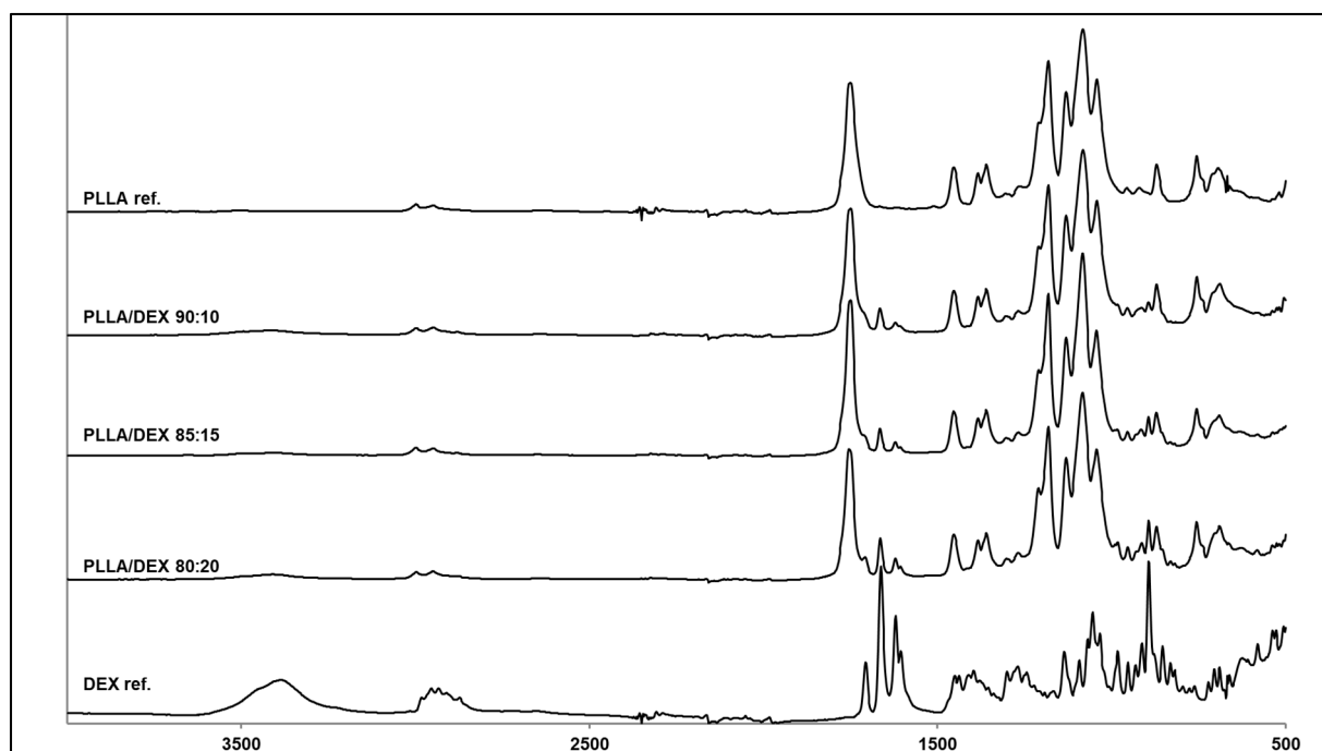
Figure S2.3: IR spectra of PLLA and PLLA with incorporated dexamethasone at 10, 15 and 20 w/w% and dexamethasone reference spectrum.
