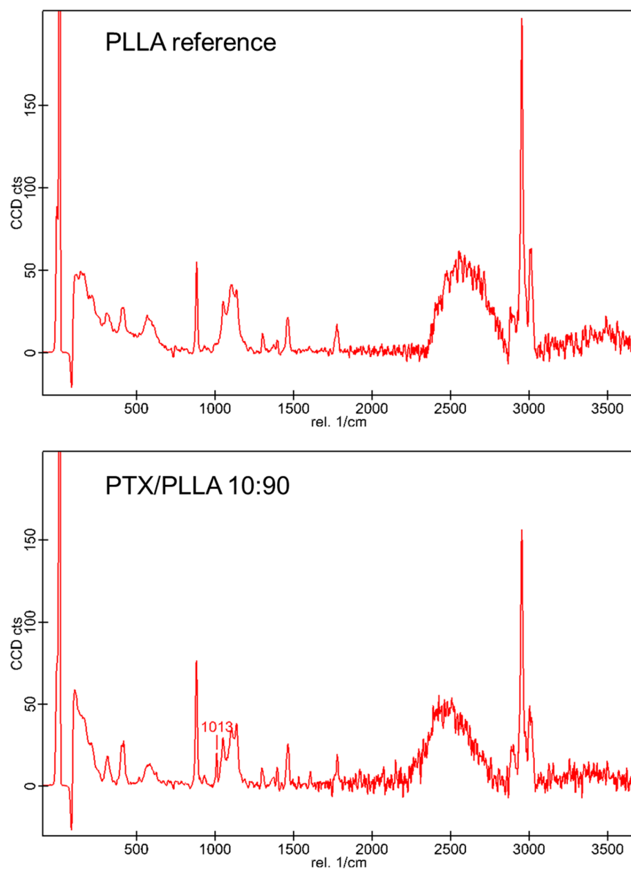
Figure S1: Raman spectra of PLLA and PLLA with incorporated drugs at a ratio of drug/PLLA = 10/90 w/w%
