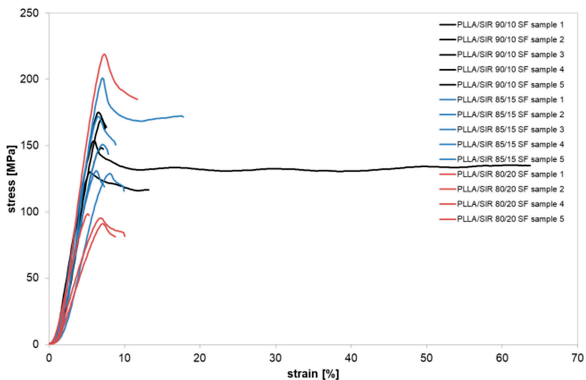
Figure S7.3: Stress strain curves of spray-coated PLLA/SIR film.
