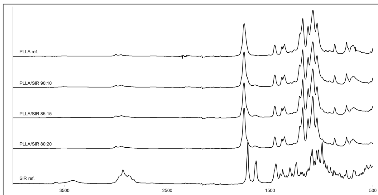
Figure S2.1: IR spectra of PLLA and PLLA with incorporated sirolimus at 10, 15 and 20 w/w% and sirolimus reference spectrum.
