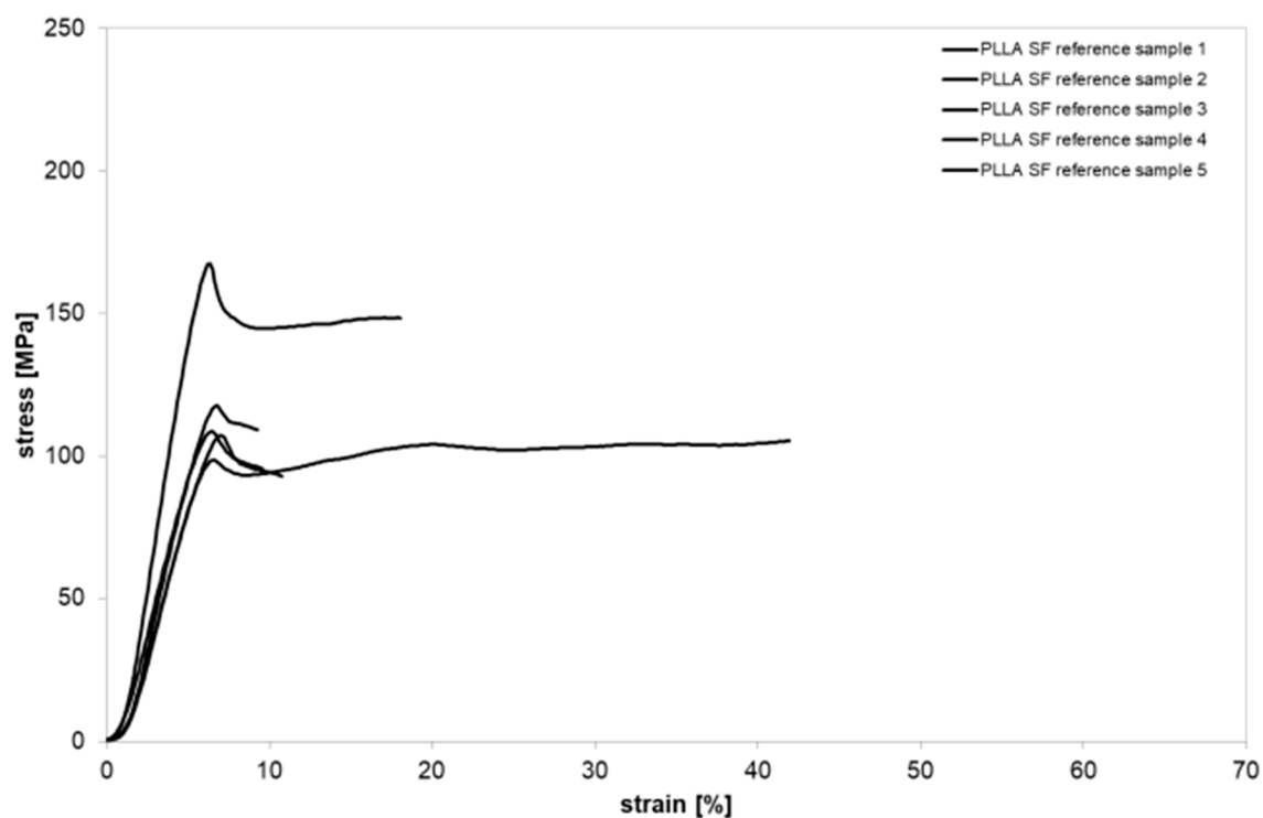
Figure S7.1: Stress strain curves of spray-coated PLLA film without any drug content.
