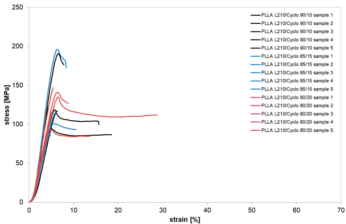
Figure S7.5: Stress strain curves of spray-coated PLLA/CICLO film.
