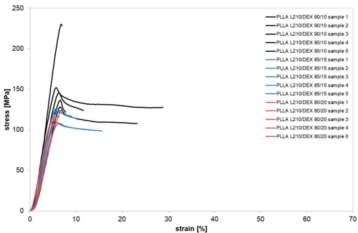
Figure S7.4: Stress strain curves of spray-coated PLLA/DEX film.
