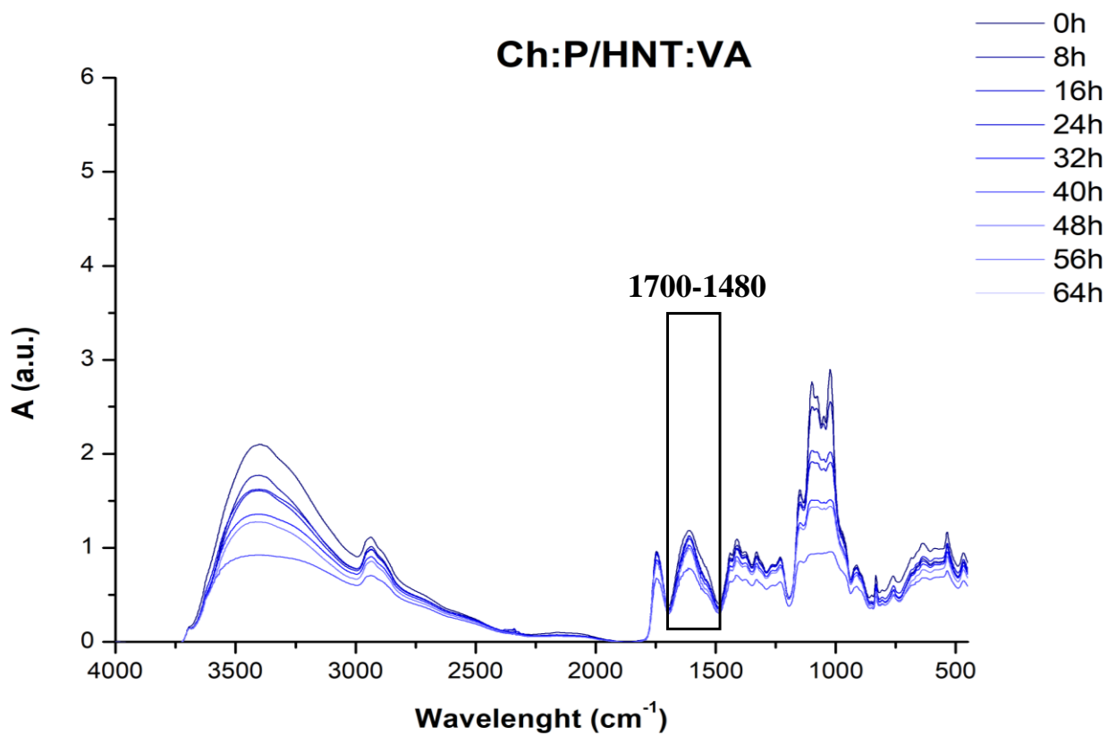
Figure S6. FTIR spectra of Ch:P/HNT:VA at different exposure time
