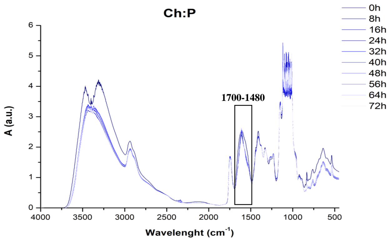
Figure S3. FTIR spectra of Ch:P at different exposure time
