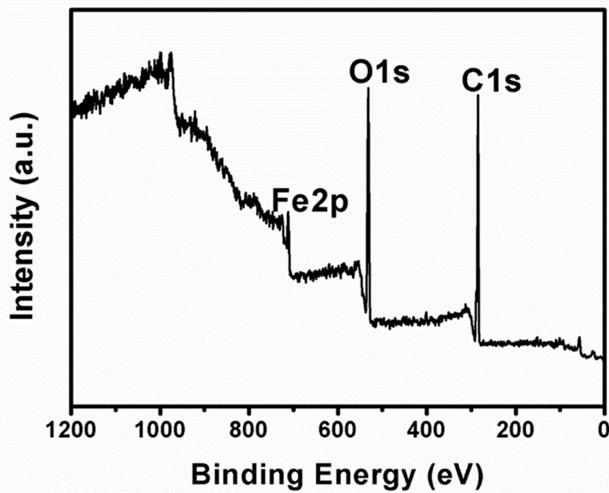
Figure S2. XPS full spectrum of MIONs@DDT-PMAA.
