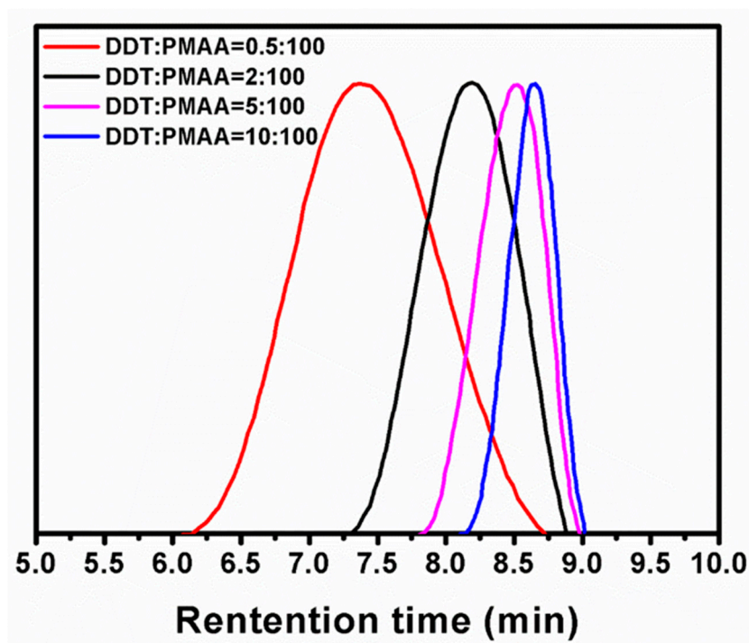
Figure S1. Normalized GPC curves of DDT-PMAA synthesized using different DDT to monomer molar ratios.
