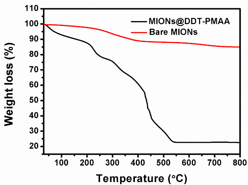
Figure S3. TGA analysis of MIONs@DDT-PMAA.
