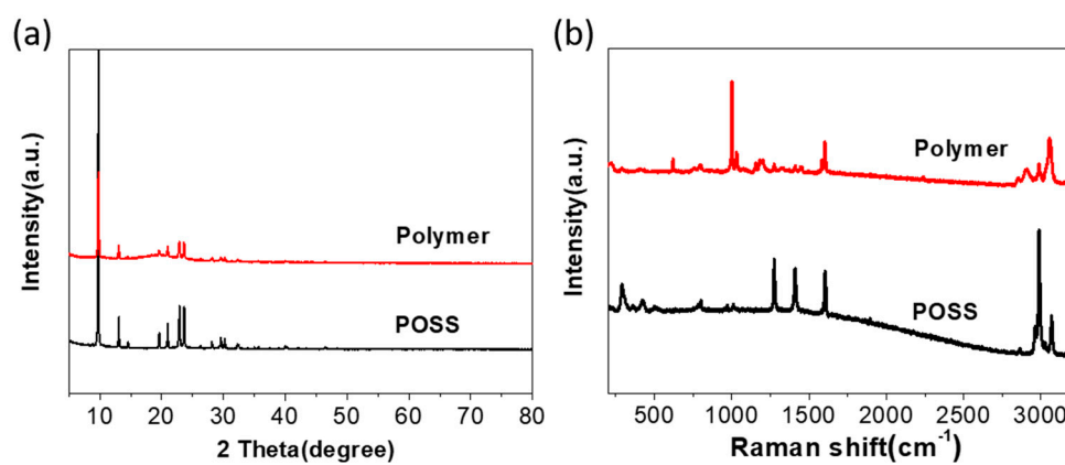
Figure.S1. (a) XRD patterns of POSS and Polymer. (b) Raman spectra of POSS and Polymer.
