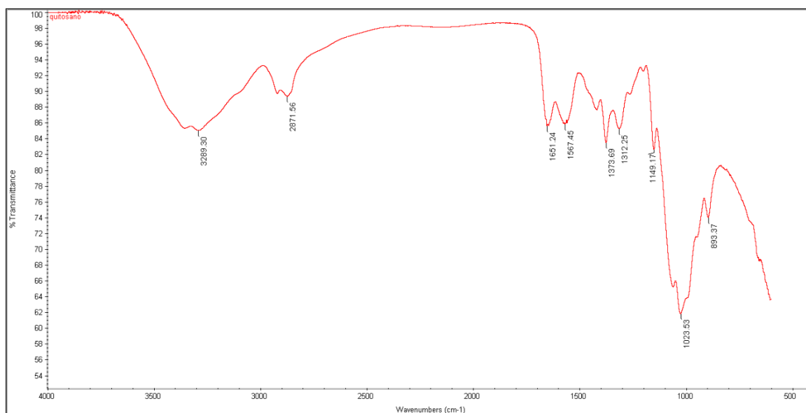
Figure S1. FTIR spectra of neat chitosan - CS
