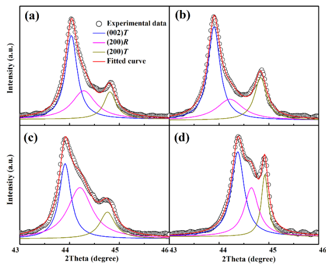
Fig. S1. Comparison of (002) T , (200) R , and (200) T reflections (from left to right) for the hard and soft PZT ceramics: (a) P4, (b) P8, (c) P5, and (d) P5H.
