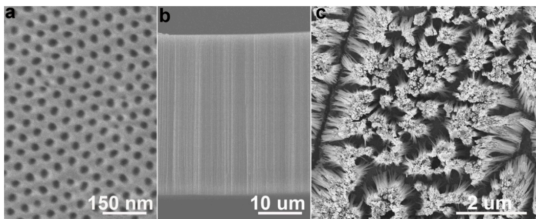
Figure 2. Typical SEM images of a AAO template: (a) plan-view, (b) view from crossing; (c) SEM image of Ni nanowire arrays (current density = 2.5 \text{ mA/cm}^2 ).
