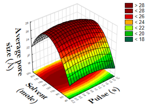
Figure S-4. Effect of ultrasound pulse and solvent on average pore size
