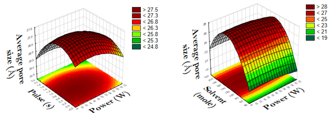
Figure S-2. Effect of ultrasound power on average pore size
