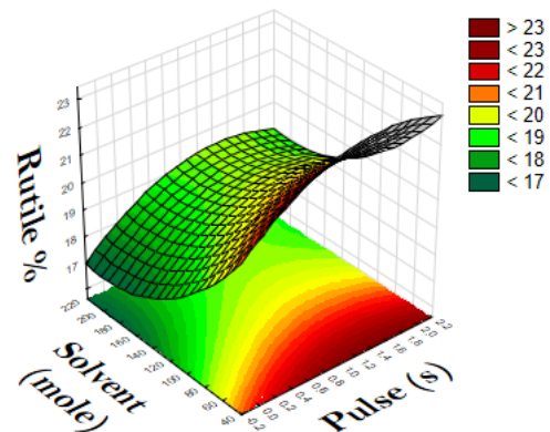
Figure S-3. Effect of ultrasound pulse and solvent on Rutile %
