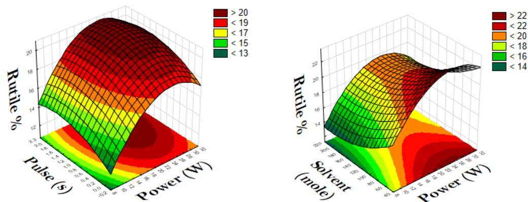
Figure S-1. Effect of ultrasound power on Rutile %
