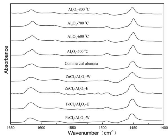
Figure S1. FTIR spectra of pyridine adsorbed on mesoporous aluminas and metal chlorides modified aluminas. Spectra are on the same scale and offset vertically for clarity.
