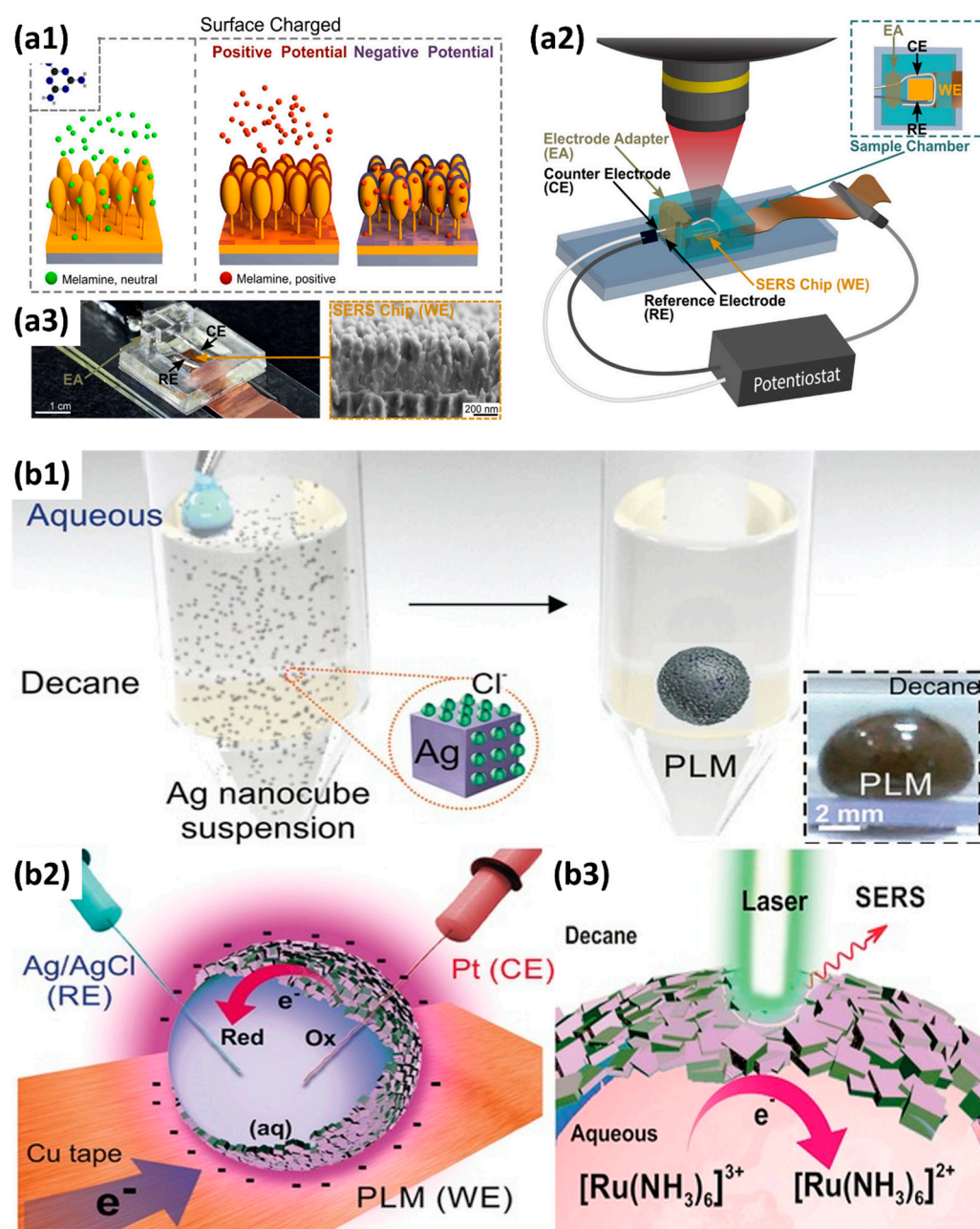
Figure 5. (a1) Schematic diagram of the electrochemically assisted SERS-based detection working principle. (a2) Illustration of the custom-made electrochemical-SERS platform and its respective system interfacing. (a3) Photo of the assembled detection chamber and SEM image of Au-capped nanopillar structures for SERS detection. Reprinted from [17], with permission from ACS Publications. (b1) Fabrication of PLM. Inset: digital image of PLM. (b2) Using the Ag shell as a 3D working electrode (WE). (b3) Electrochemistry-SERS investigation using PLM. Reprinted from [20], with permission from John Wiley and Sons.
