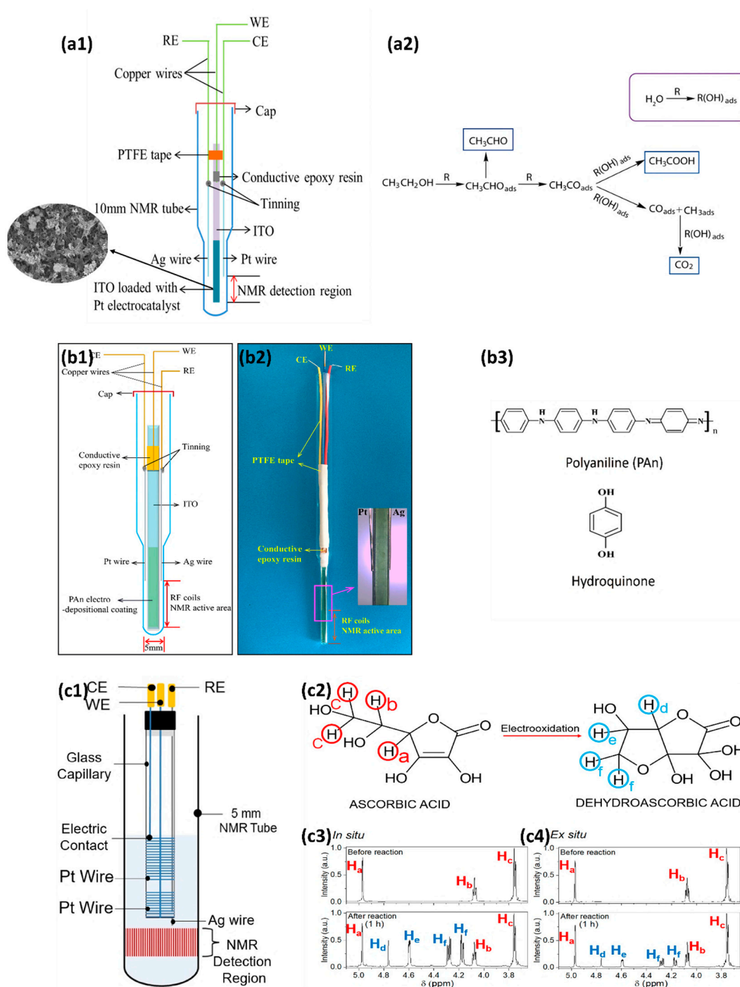
Figure 6. (a1) Schematic structure of the electrochemical cell designed for in situ EC-NMR experiment. (a2) Reaction mechanism of ethanol oxidation on Pt/MoS 2 /GNS. Reprinted from [77], with permission from Elsevier. (b1,b2) Electrochemical cell designed for in situ EC-NMR; (b3) The molecular structure of polyaniline (PAN) and hydroquinone (QH 2 ). Reprinted from [11], with permission from Elsevier. (c1) Electrochemical cell and electrodes. The WE, CE, and RE are fixated on the glass capillary tube. (c2) The different hydrogen atoms observed in the NMR spectra are highlighted. In addition, the 1 H NMR spectra of the oxidation of ascorbic acid in situ (c3) and ex situ (c4) are shown. Reprinted from [78], with permission from Elsevier.
