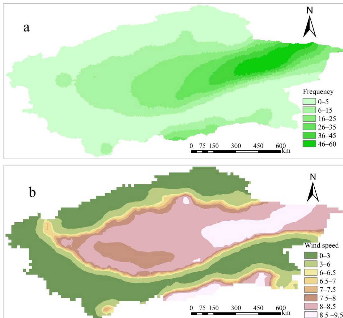
Figure 10. (a) Gale weather frequency; (b) Annual average wind speed in gale weather.
