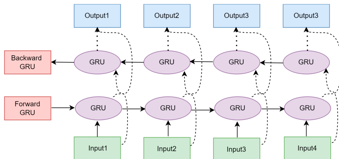
Figure 3. Bidirectional Gated Recurrent Unit.
