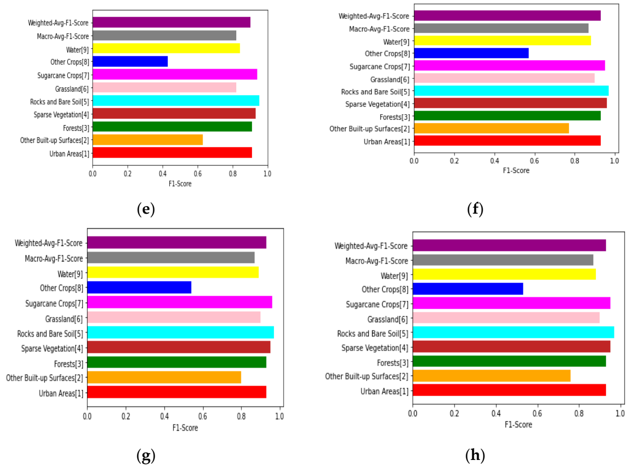
Figure 7. F1 scores of land cover classification for the time series dataset using the deep learning model: (a) bidirectional GRU; (b) temporal CNN; (c) GRU + temporal CNN; (d) attention on temporal CNN; (e) attention on temporal CNN + GRU; (f) univariate + multivariate + coordinates; (g) univariate + multivariate; (h) univariate + multivariate (LSTM) + coordinates.
