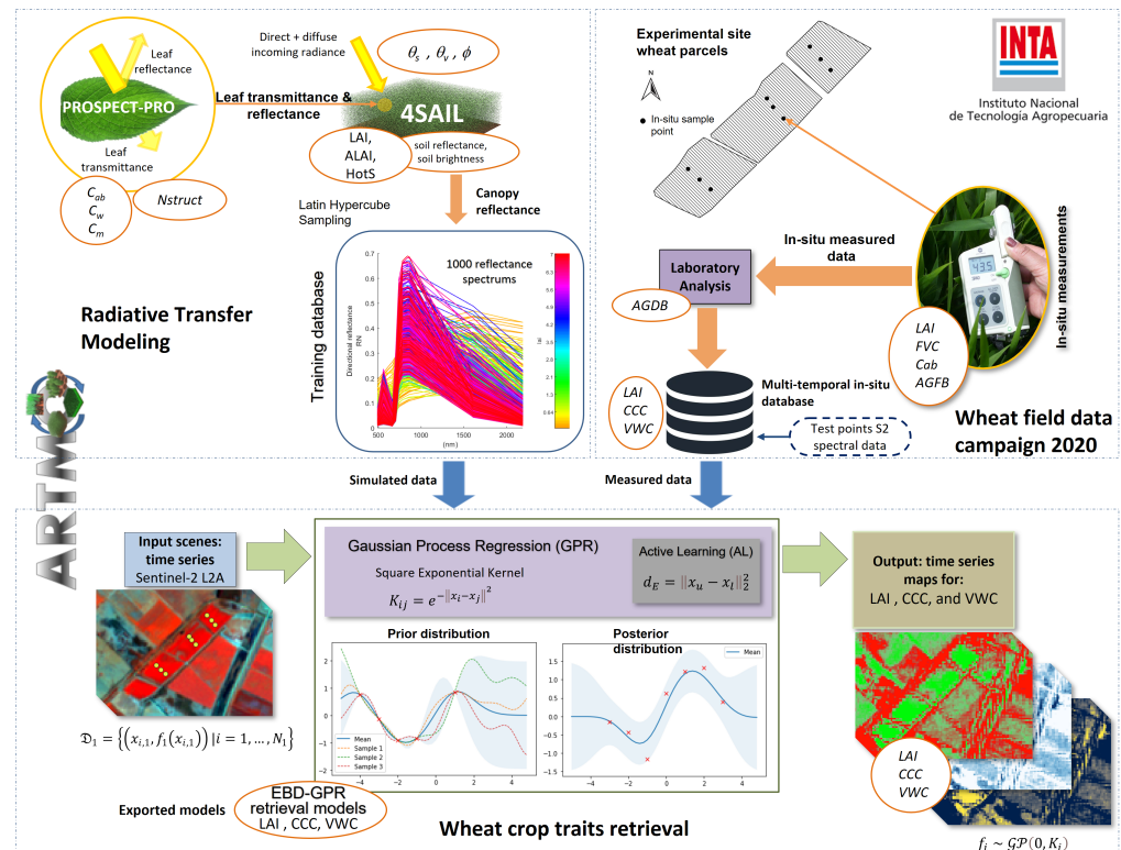
Figure 4. Illustration of the hybrid retrieval workflow using the coupled PROSAIL-PRO models to establish a training database for the GPR, partly adapted from [82]. The output maps show our vegetation traits modeling over the BVCR area in Argentina.
