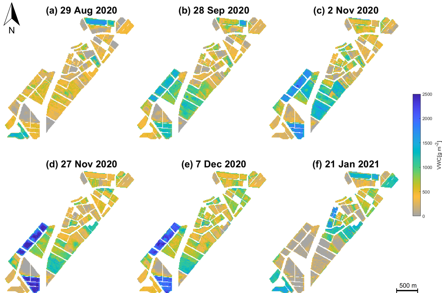
Figure 9. VWC [g m -2 ] of different crops in the study site, retrieved by the GPR model using simulated vegetation reflectance spectra, in-situ biophysical/biochemical measurements and S2 surface multi-spectral reflectance data. Data obtained from BVCR wheat campaign 2020. (a) wheat tillering stage at 29 August 2020; (b) wheat booting stage at 28 September 2020; (c) wheat anthesis-flowering stage at 2 November 2020; (d) wheat dough development stage at 27 November 2020; (e) wheat ripening stage at 7 December 2020; (f) harvested wheat at 21 January 2021.
