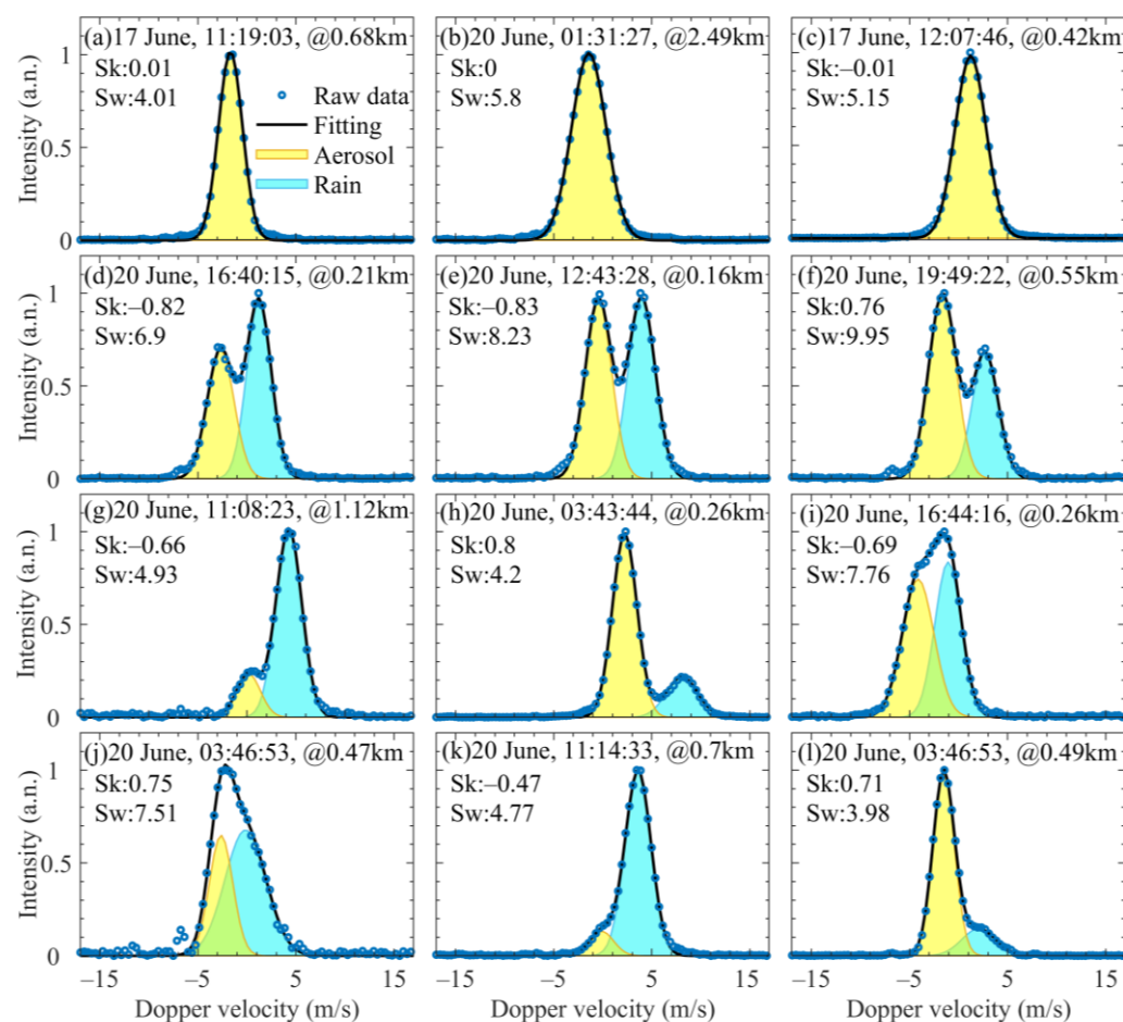
Figure 3. Examples of different types of Doppler spectra. (a) General aerosol spectrum; (b) cloud spectrum; (c) spectrum under strong turbulence; (d–l) precipitation spectra and its separation results. Circles stand for the raw data of spectra. Black lines represent fitting results. The yellow shadow and light blue shadow represent separated aerosol and rain components, respectively.
