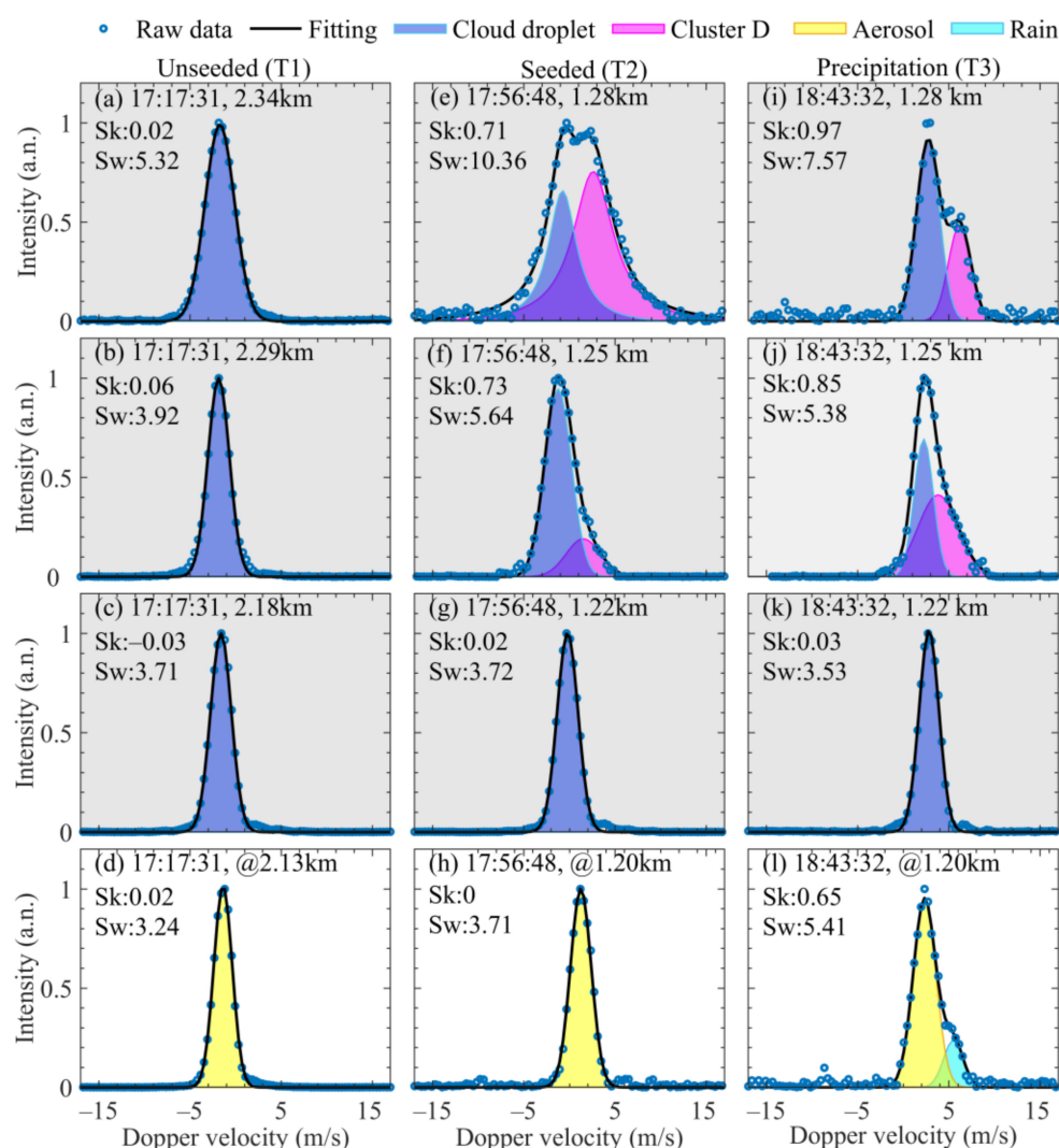
Figure 9. Examples of cloud spectra from cloud middle to cloud base. (a–c) show cloud spectra of unseeded at T1 (5:17 p.m.); (e–g) show cloud spectra of after seeded at T2 (5:56 p.m.); (i–k) show cloud spectra at T3 (6:43 p.m.), when precipitation formed. (d,h,l) are aerosol or precipitation spectra below cloud base. Circles stand for the raw data of spectra. Black lines represent fitting results. The light purple shadow and pink shadow represent separated cloud droplet and cluster D, respectively. The yellow shadow and light blue shadow represent separated aerosol and rain components, respectively.
