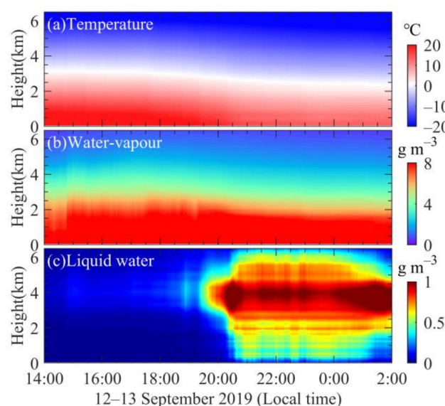
Figure 5. Continuous MWR observation results during 12–13 September 2019.
