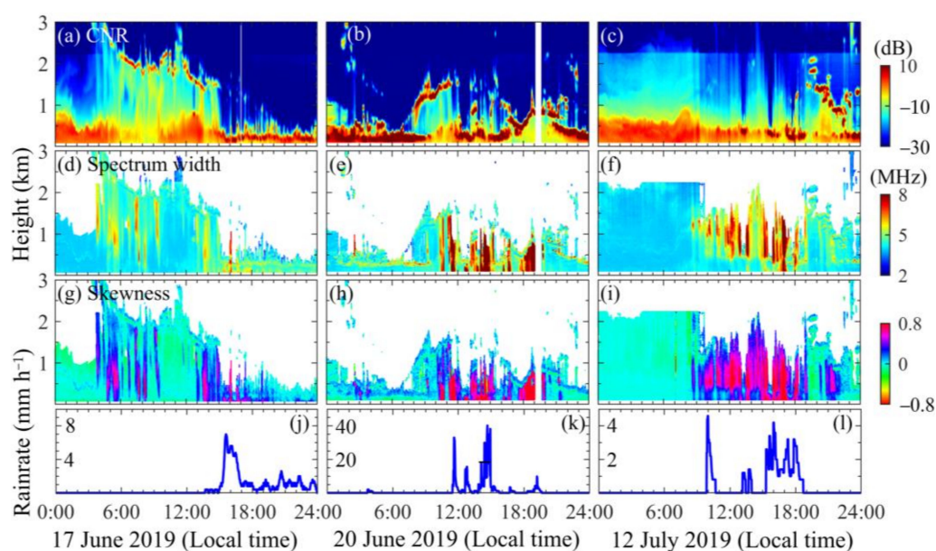
Figure 1. Precipitation processes observed by the CDWL on 17 June 2019, 20 June 2019, and 12 July 2019. (a–c) CNR. (d–f) spectrum width. (g–i) skewness. (j–l) surface rain rate provided by a Davis weather station.
