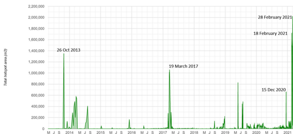
Figure 8. Plot of hotspot area generated through the NHI tool, integrating L8-OLI (from April 2013 onwards) and S2-MSI observations (from June 2015 onwards).
