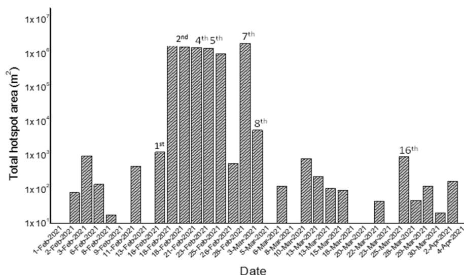
Figure 4. Temporal trend of the total hotspot area (m 2 ) retrieved using NHI tool, by integrating L8-OLI and S2-MSI observations over the period 1 February–4 April 2021, with the indication of the relative paroxysm.
