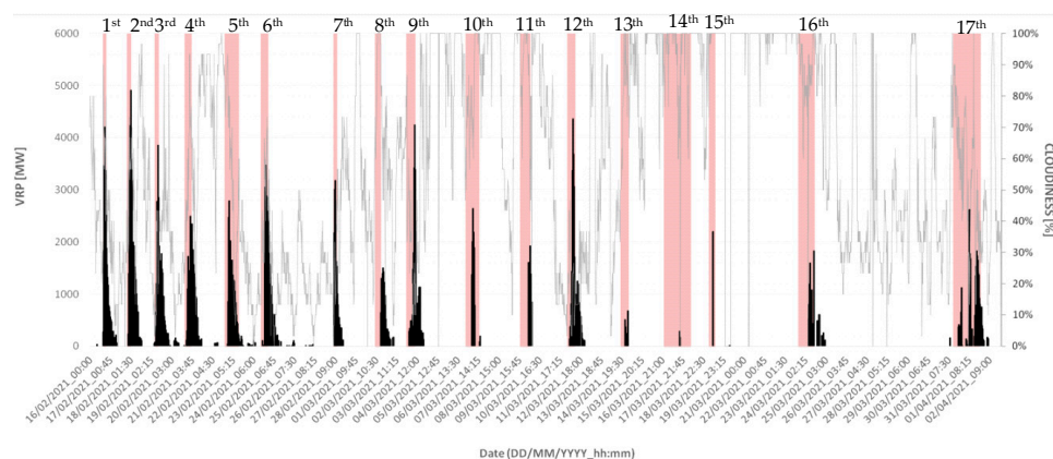
Figure 7. Temporal trend of VRP retrieved from SEVIRI (in black) data (at 15 min time interval) starting from RST VOLC detections with the indication of the number of the Mt. Etna paroxysms. Paroxysms’ time duration (light pink bars) and cloudiness percentage (light grey line) are represented as well.
